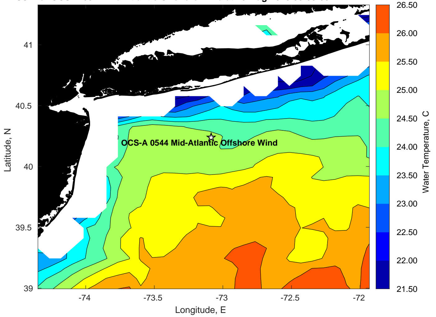
SST for OCS-A 0544 Mid-Atlantic Offshore Wind at 15-Aug-2023 00:00:00
