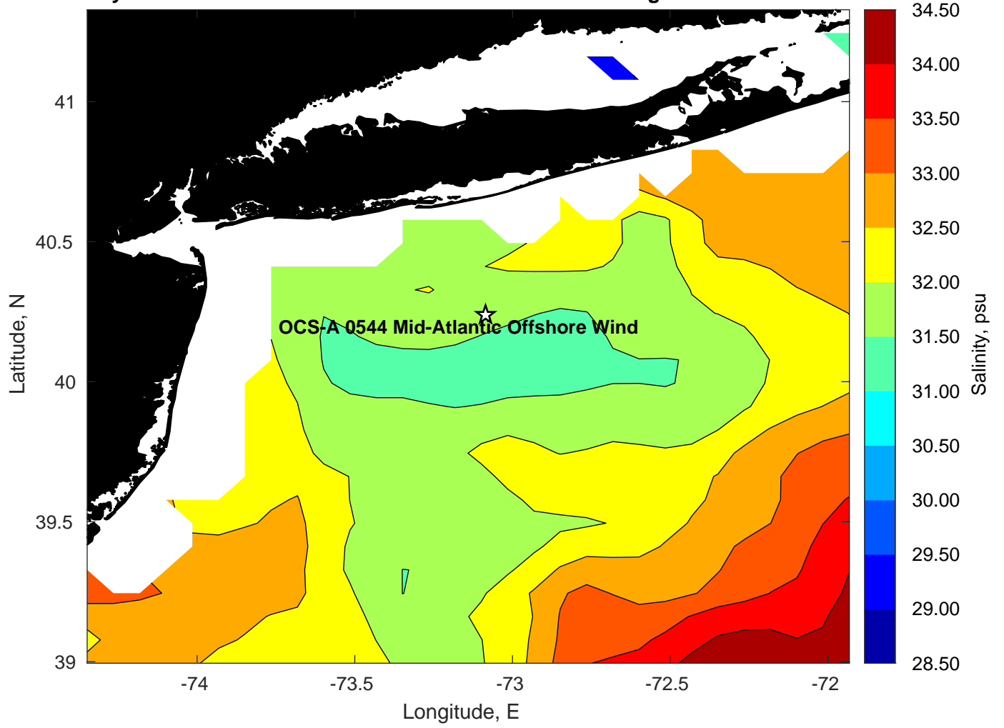
Surface Salinity for OCS-A 0544 Mid-Atlantic Offshore Wind at 15-Aug-2023 00:00:00
