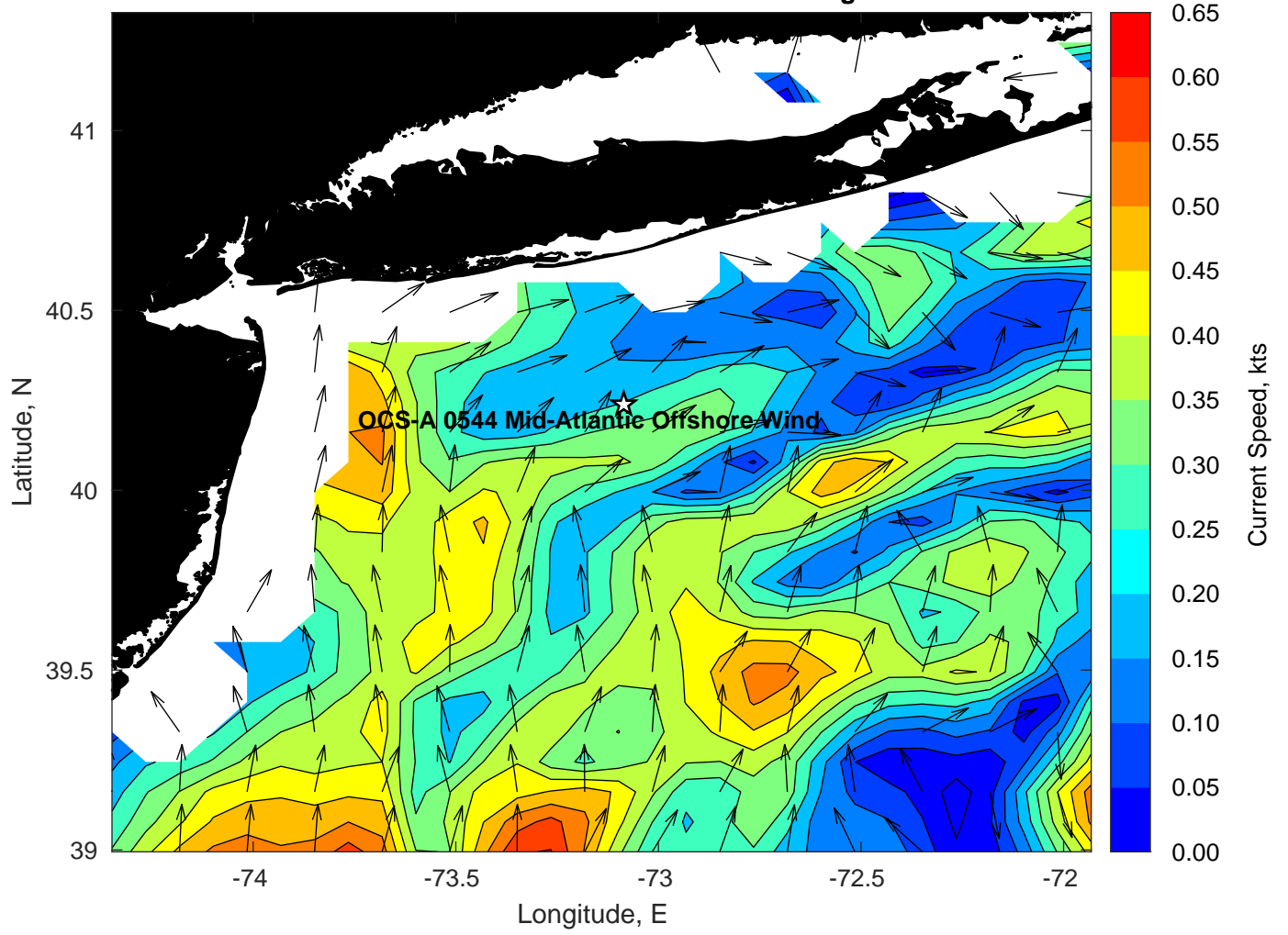
Surface Currents for OCS-A 0544 Mid-Atlantic Offshore Wind at 15-Aug-2023 00:00:00
