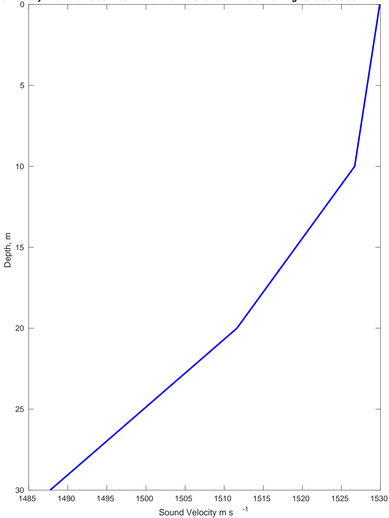
Sound Velocity Profile for OCS-A 0544 Mid-Atlantic Offshore Wind on 15-Aug-2023 00:00:00
