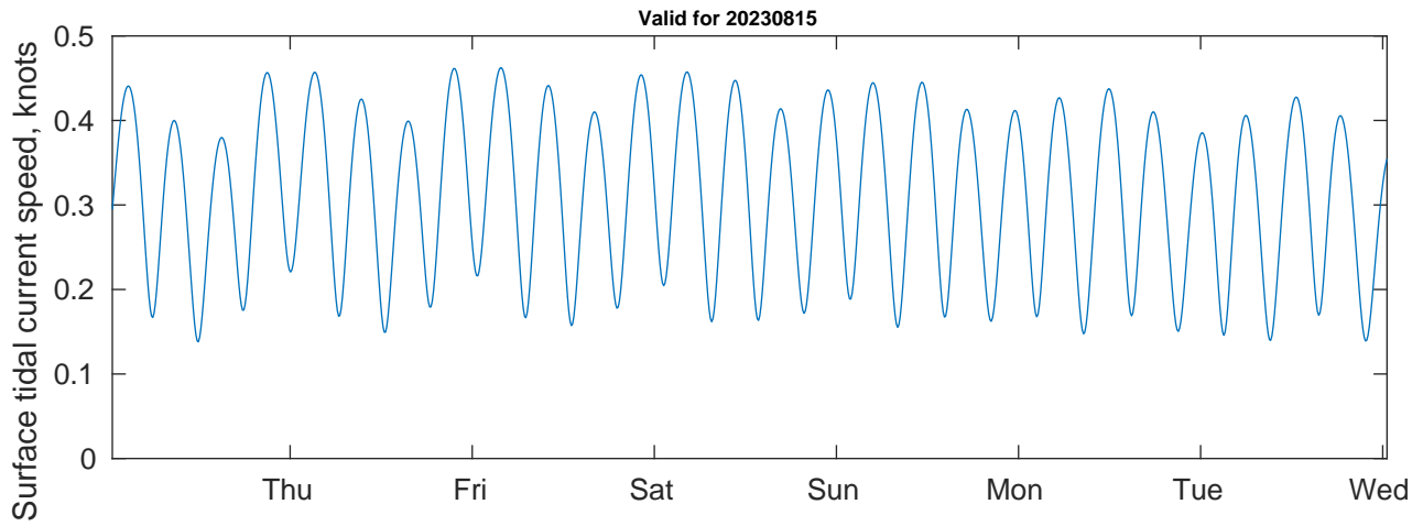
Tidal Currents and Heights for OCS-A 0544 Mid-Atlantic Offshore Wind at 20230815
