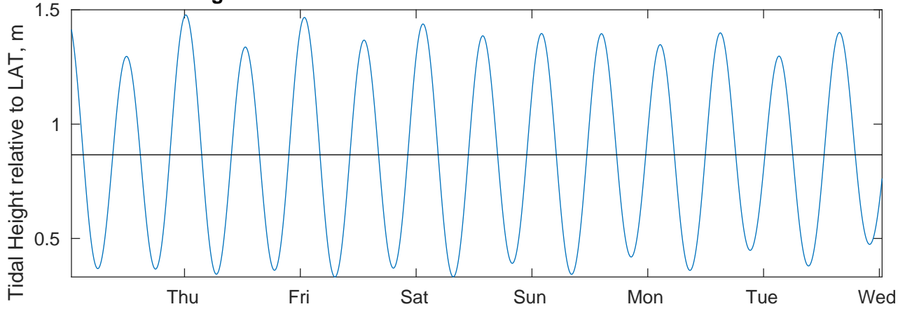
Tidal Currents and Heights for OCS-A 0544 Mid-Atlantic Offshore Wind at 20230815
