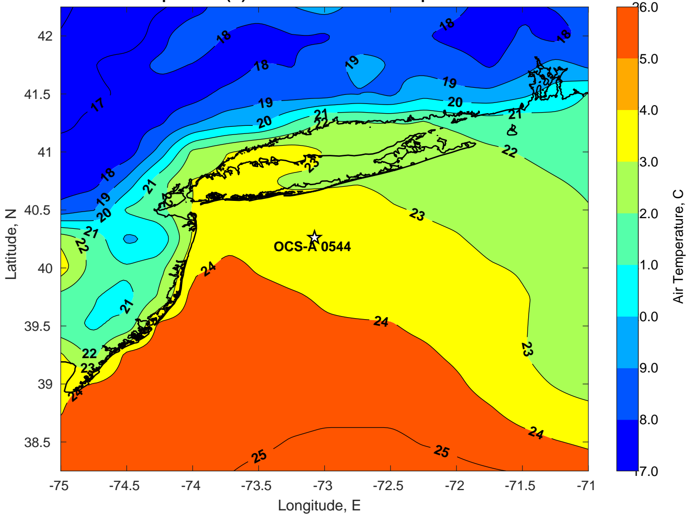
Air Temperature (C) for OCS-A 0544 at 21-Sep-2022
