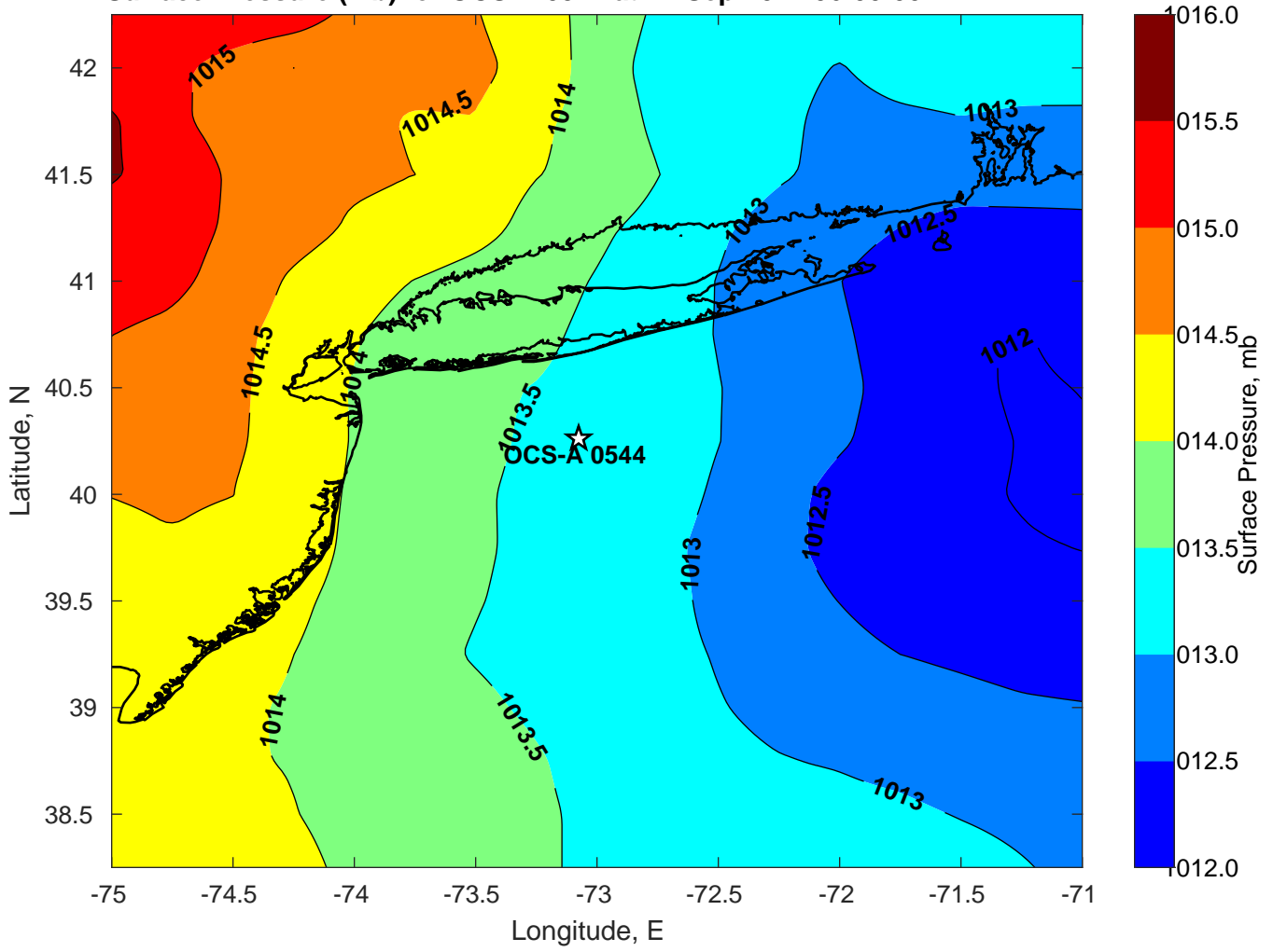
Surface Pressure (mb) for OCS-A 0544 at 21-Sep-2022 06:00:00
