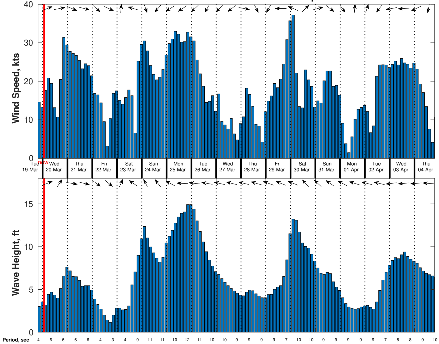
Wind & Wave Forecast for OCS-A 0544 from 19-Mar-2024 19:00:00 to 04-Apr-2024 19:00:00
