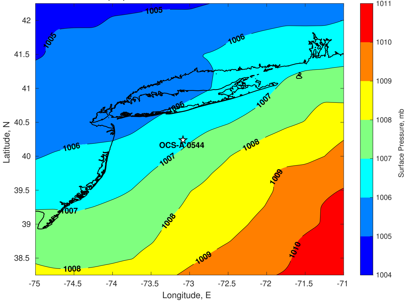
Surface Pressure (mb) for OCS-A 0544 at 20-Mar-2024 06:00:00
