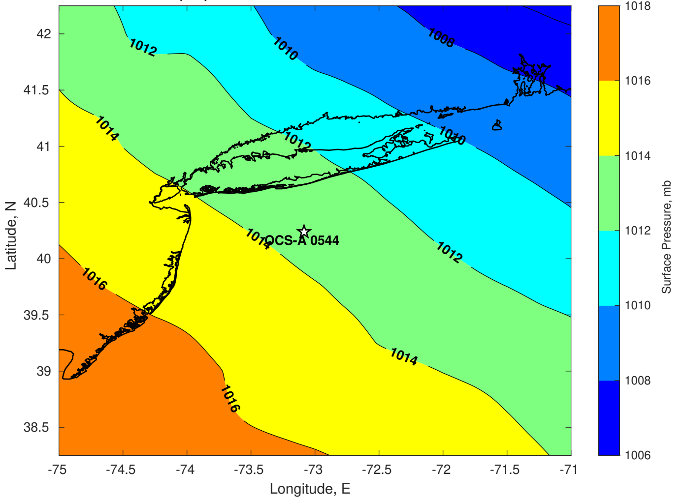
Surface Pressure (mb) for OCS-A 0544 at 21-Mar-2024 06:00:00
