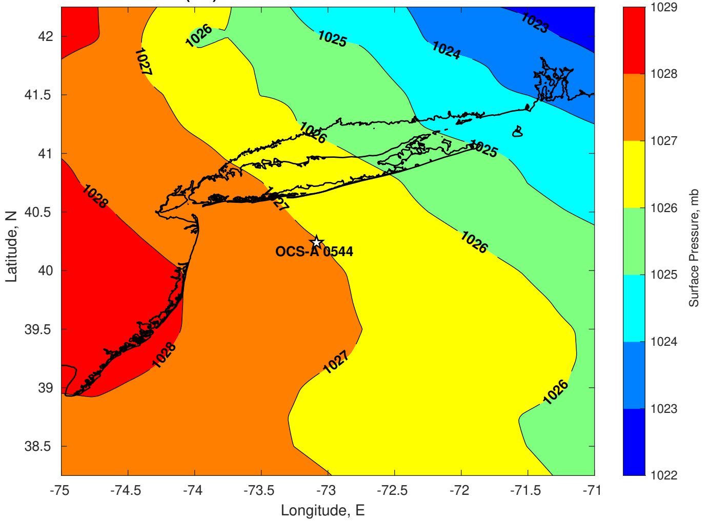
Surface Pressure (mb) for OCS-A 0544 at 22-Mar-2024 06:00:00
