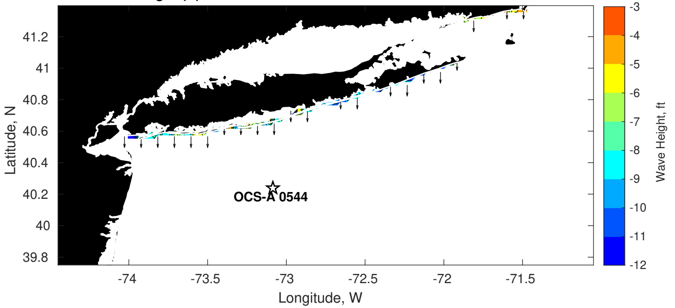
Wave Height (ft) for OCS-A 0544 at 20-Mar-2024 11:00:00
