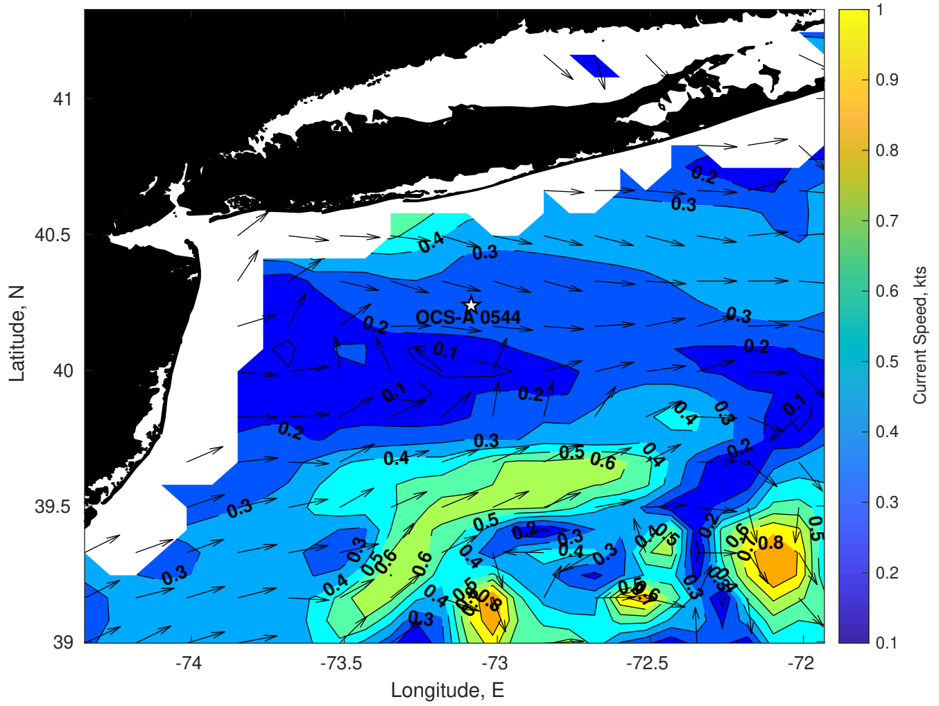
Surface Currents for OCS-A 0544 at 20-Mar-2024 00:00:00
