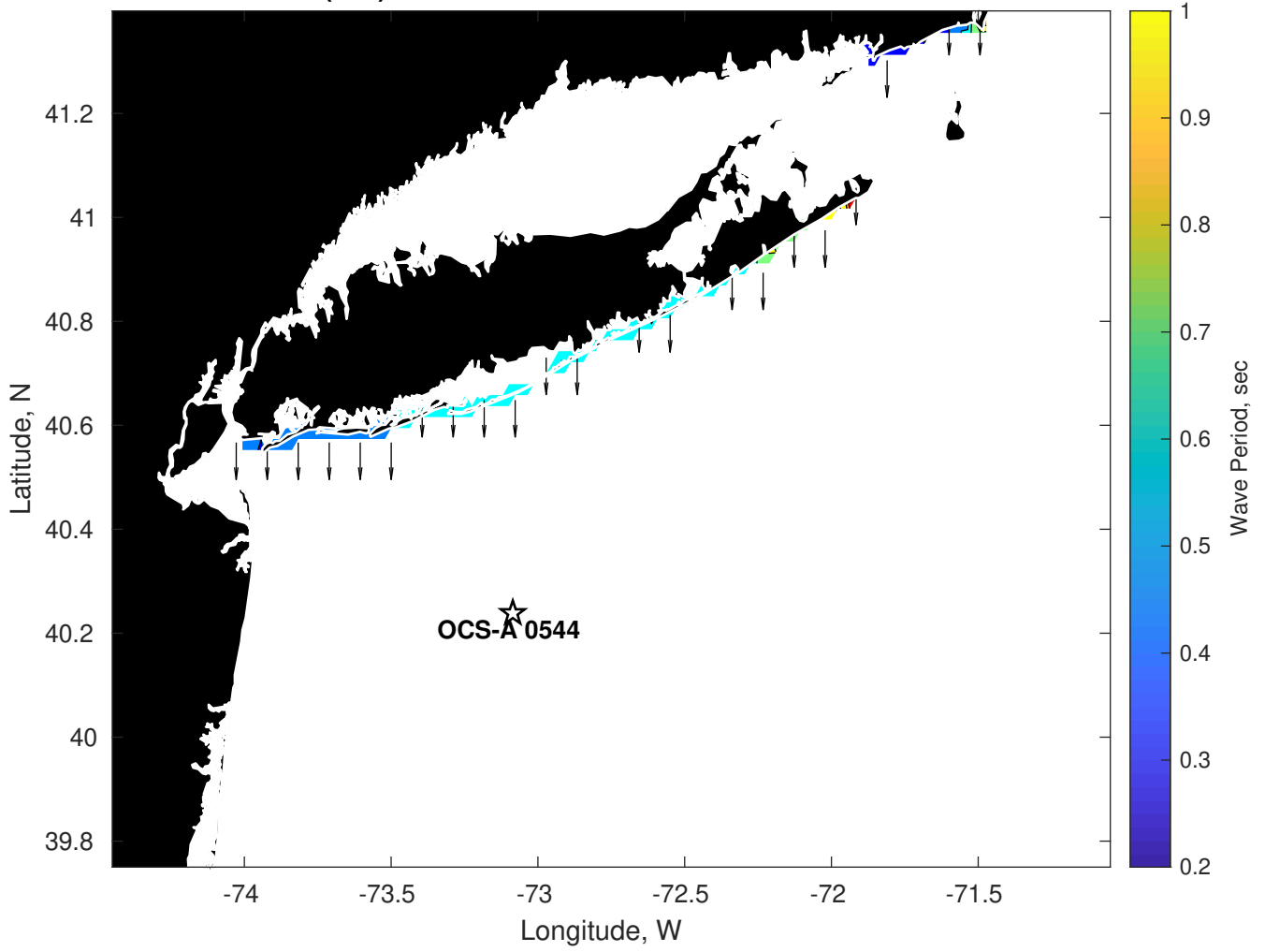
Wave Period (sec) for OCS-A 0544 at 20-Mar-2024 11:00:00
