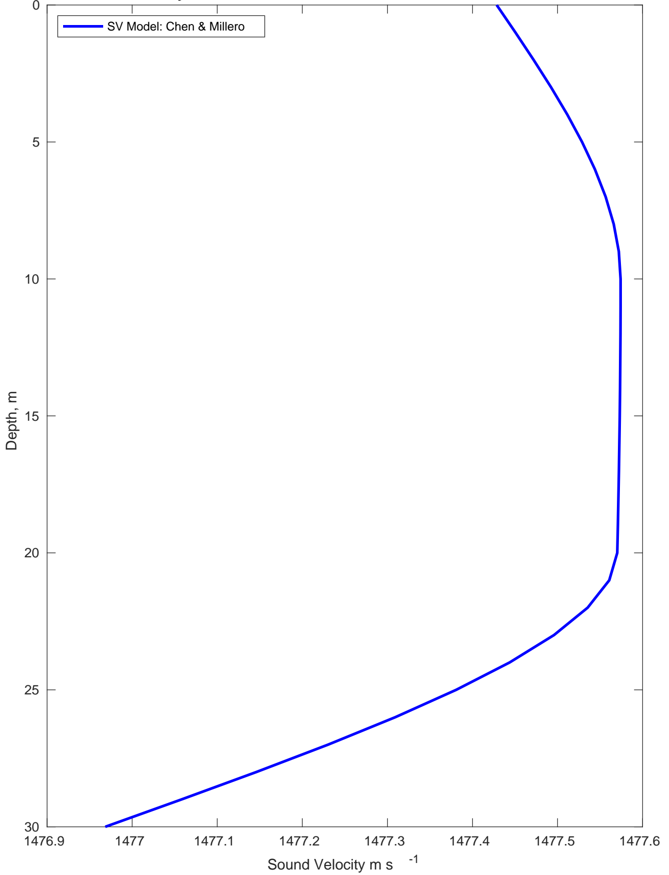
Sound Velocity Profile for OCS-A 0544 on 20-Mar-2024 00:00:00
