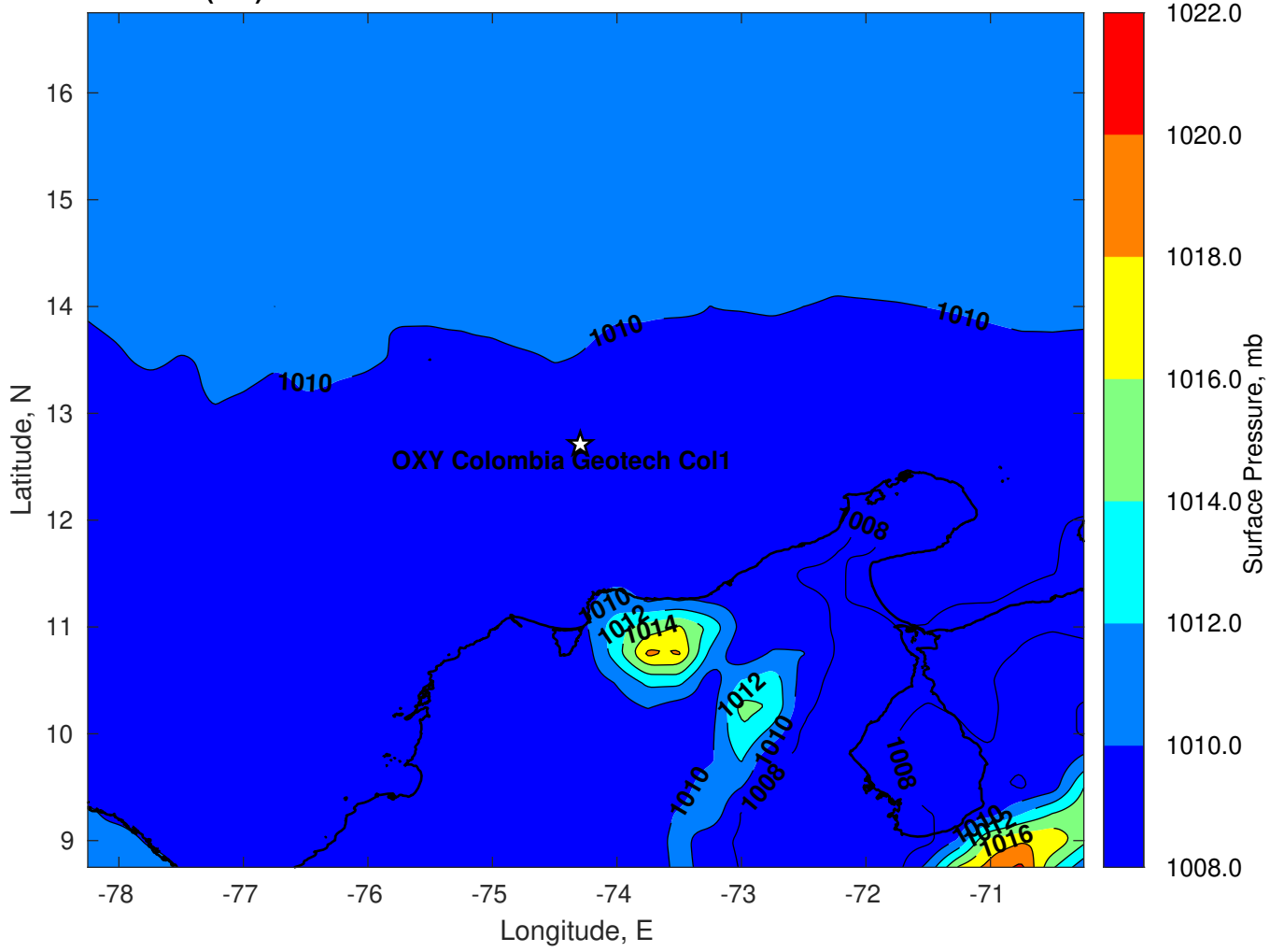
Surface Pressure (mb) for OXY Colombia Geotech Col1 at 16-Oct-2023 18:00:00
