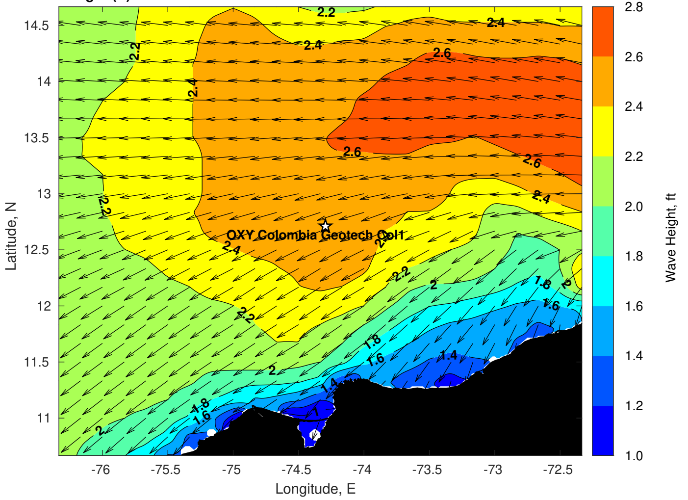
Wave Height (ft) for OXY Colombia Geotech Col1 at 15-Oct-2023 18:00:00
