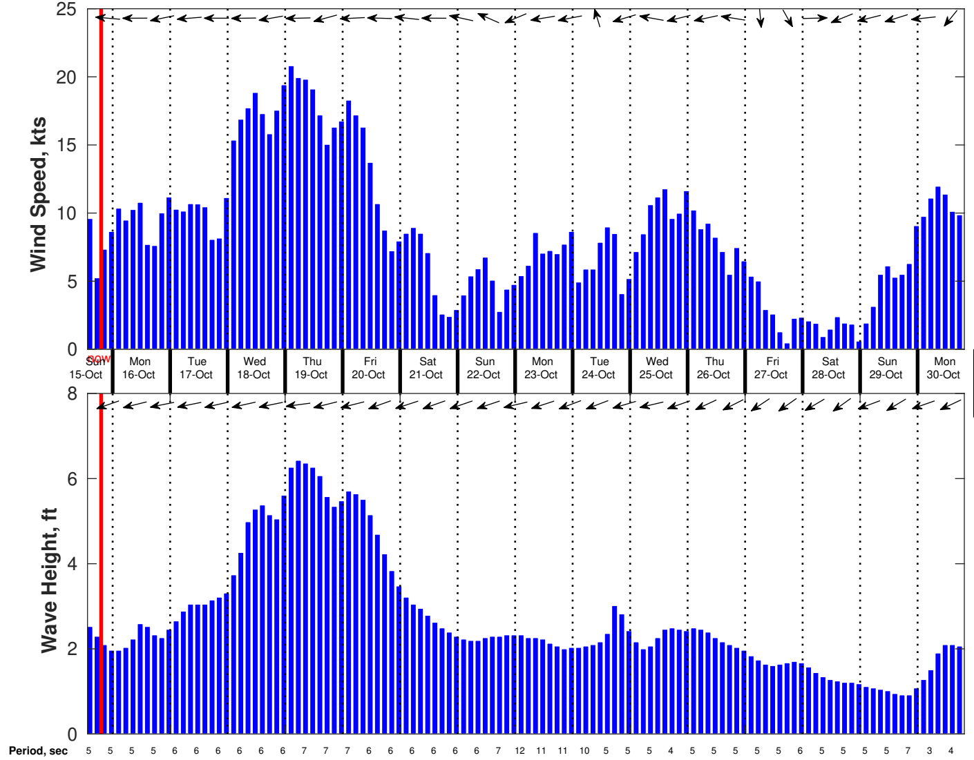
Wind & Wave Forecast for OXY Colombia Geotech Col1 from 15-Oct-2023 13:00:00 to 31-Oct-2023 13:00:00
