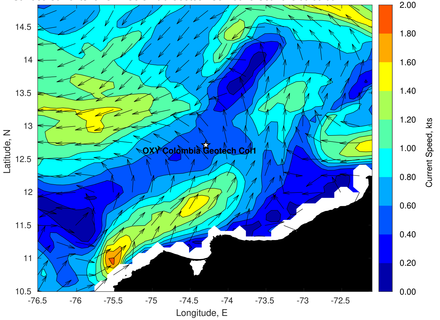
Surface Currents for OXY Colombia Geotech Col1 at 15-Oct-2023 00:00:00
