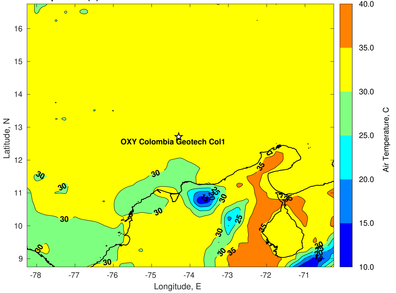
Air Temperature (C) for OXY Colombia Geotech Col1 at 15-Oct-2023
