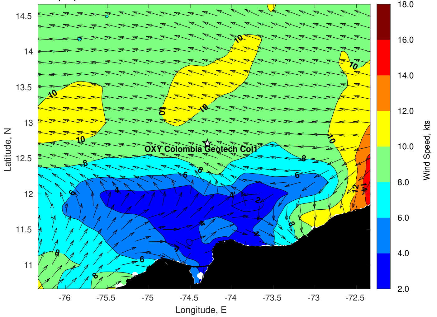
Winds (kts) for OXY Colombia Geotech Col1 at 15-Oct-2023 18:00:00
