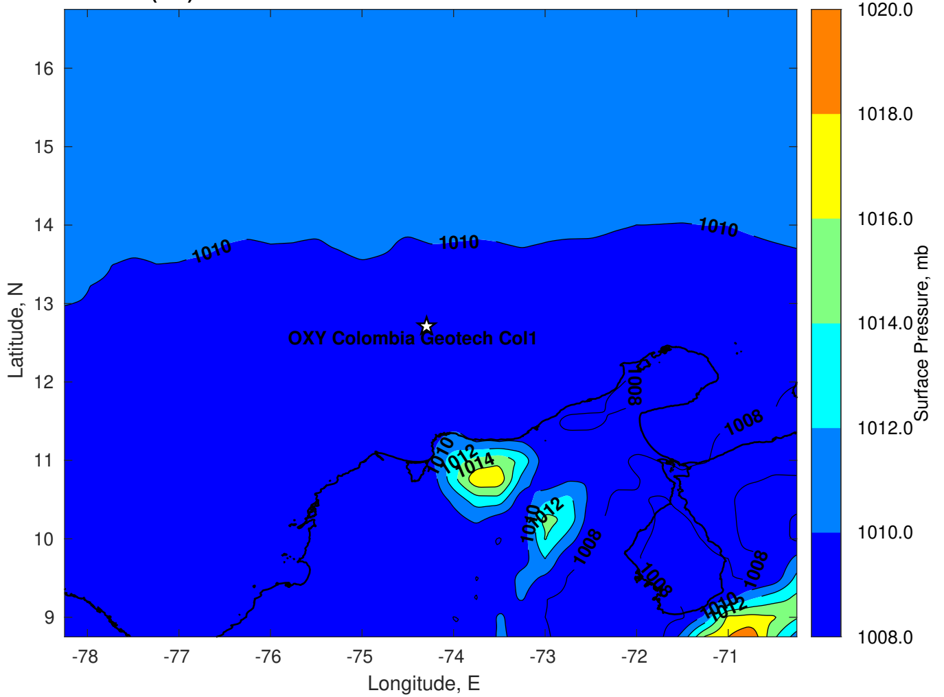
Surface Pressure (mb) for OXY Colombia Geotech Col1 at 15-Oct-2023 18:00:00
