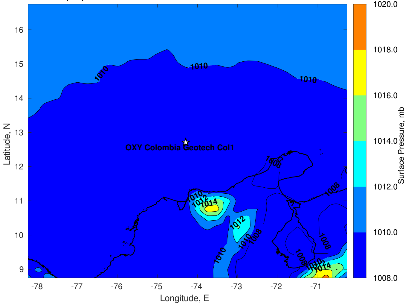
Surface Pressure (mb) for OXY Colombia Geotech Col1 at 17-Oct-2023 18:00:00
