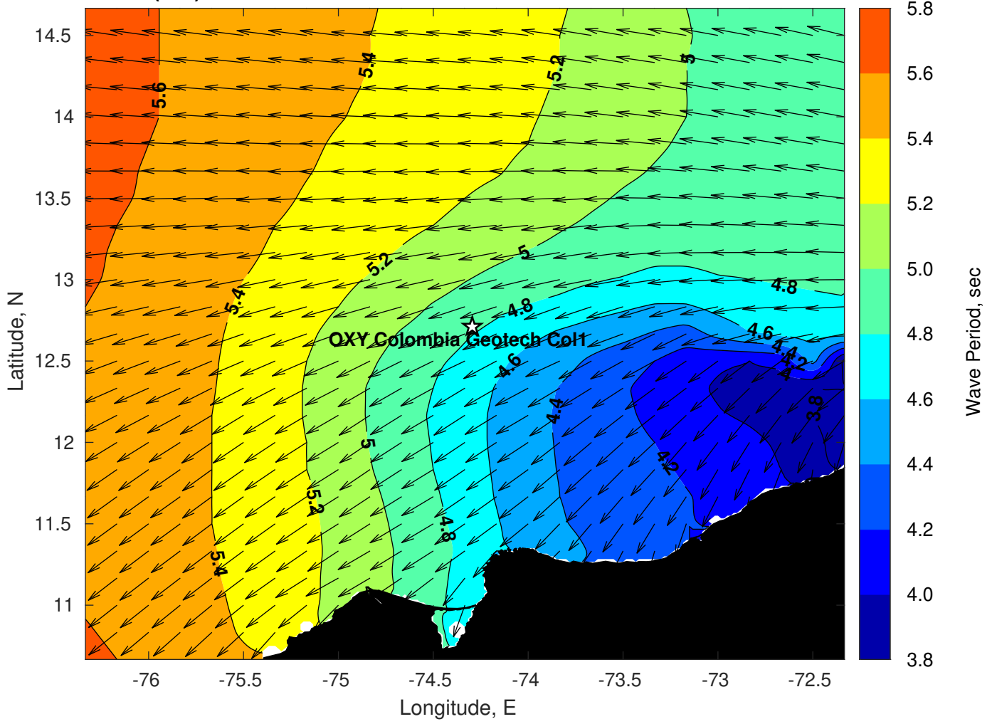
Wave Period (sec) for OXY Colombia Geotech Col1 at 15-Oct-2023 18:00:00
