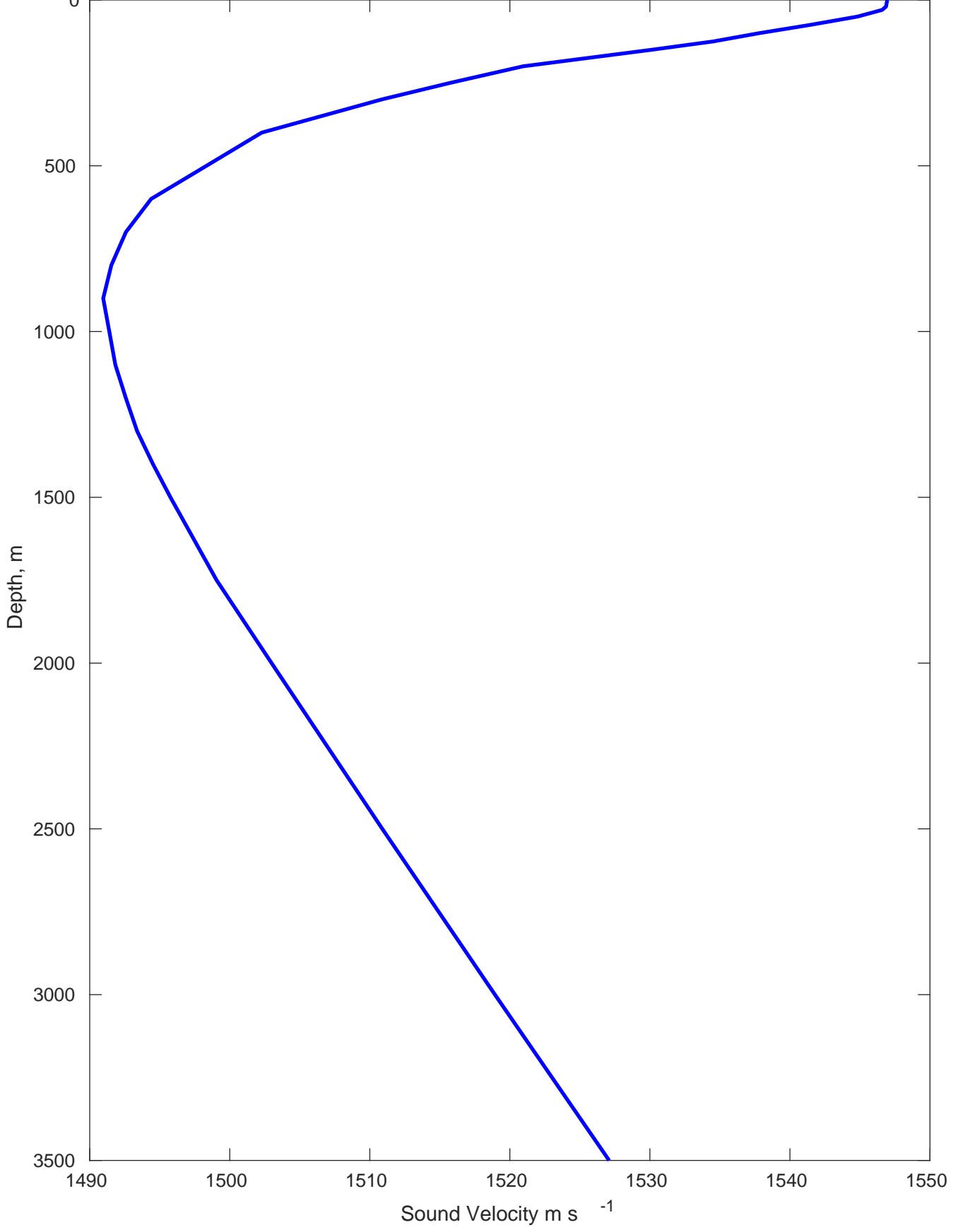
Sound Velocity Profile for OXY Colombia Geotech Co11 on 15-Oct-2023 00:00:00
