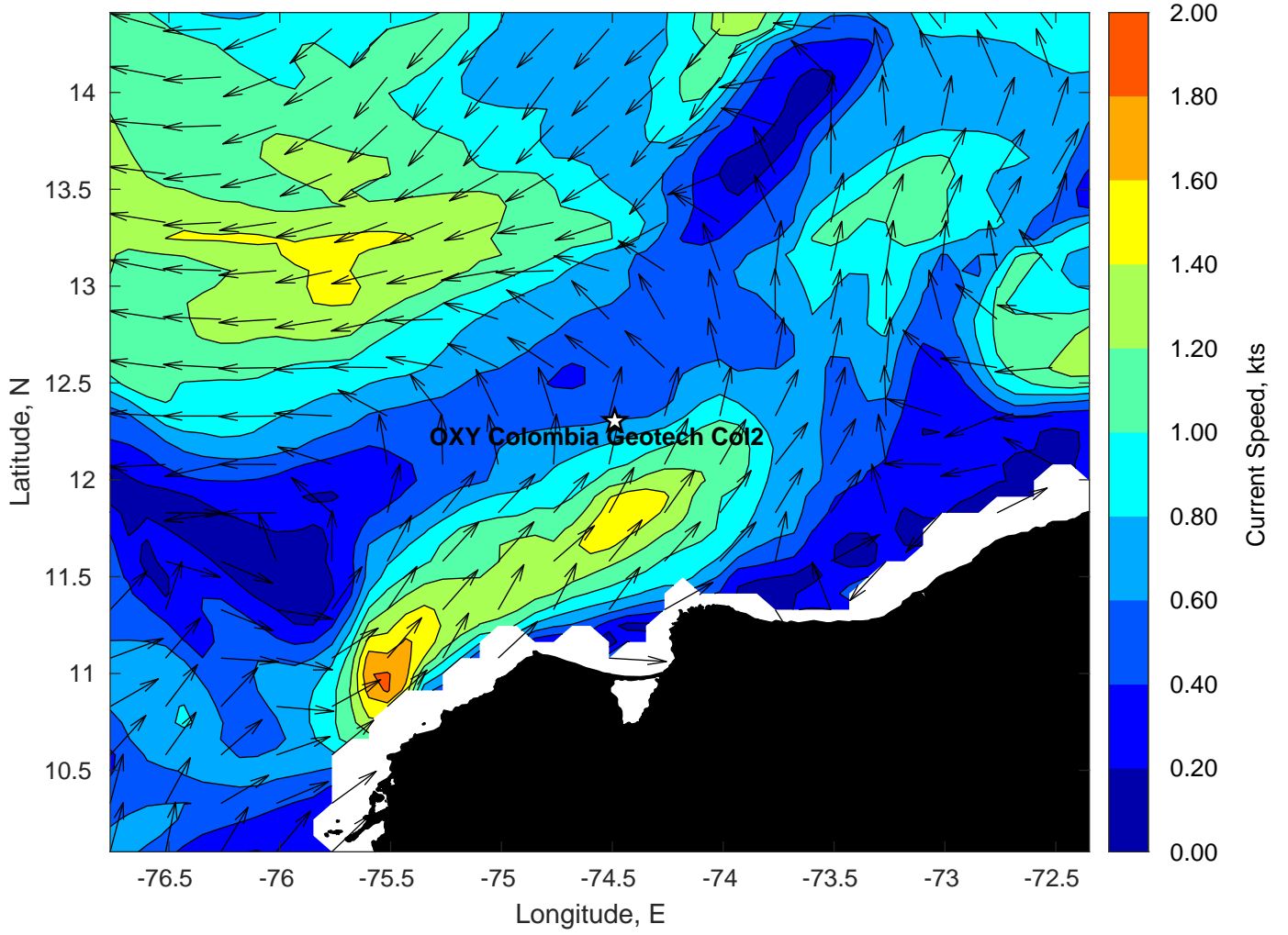
Surface Currents for OXY Colombia Geotech Col2 at 15-Oct-2023 00:00:00
