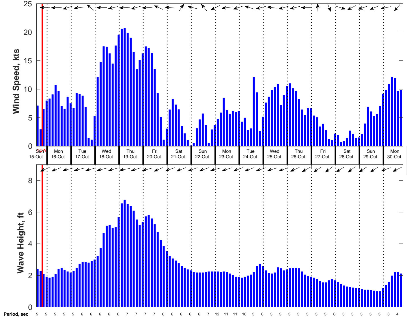
Wind & Wave Forecast for OXY Colombia Geotech Col2 from 15-Oct-2023 13:00:00 to 31-Oct-2023 13:00:00
