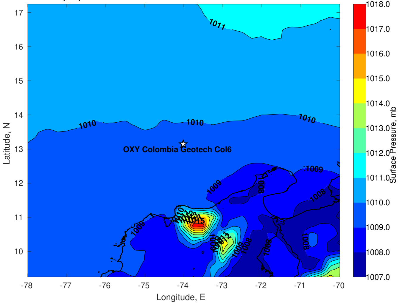
Surface Pressure (mb) for OXY Colombia Geotech Col6 at 15-Oct-2023 18:00:00
