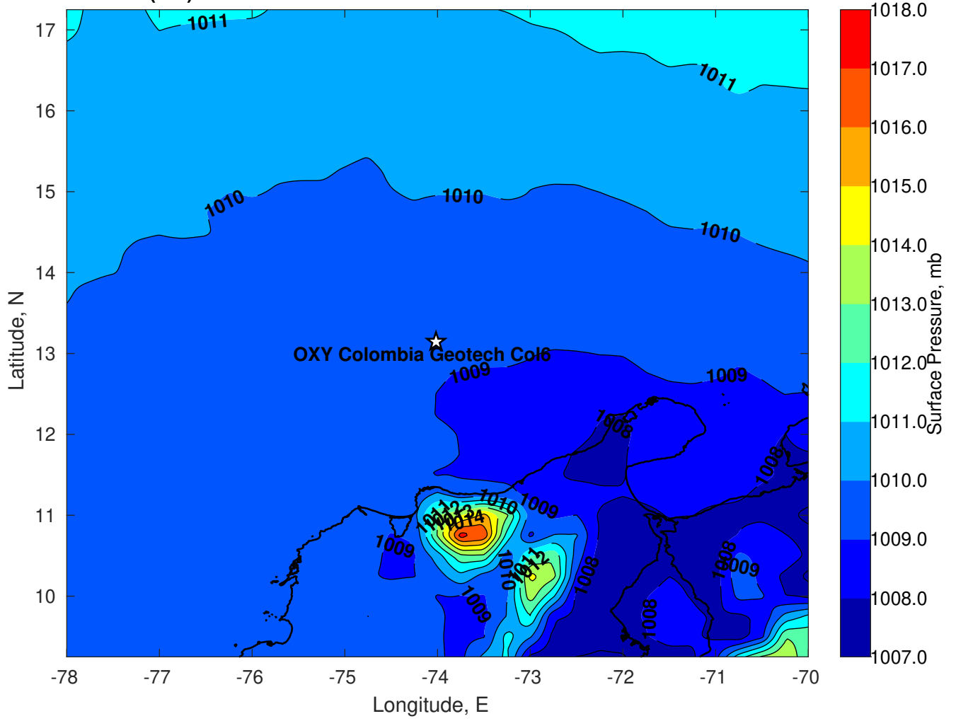
Surface Pressure (mb) for OXY Colombia Geotech Col6 at 17-Oct-2023 18:00:00
