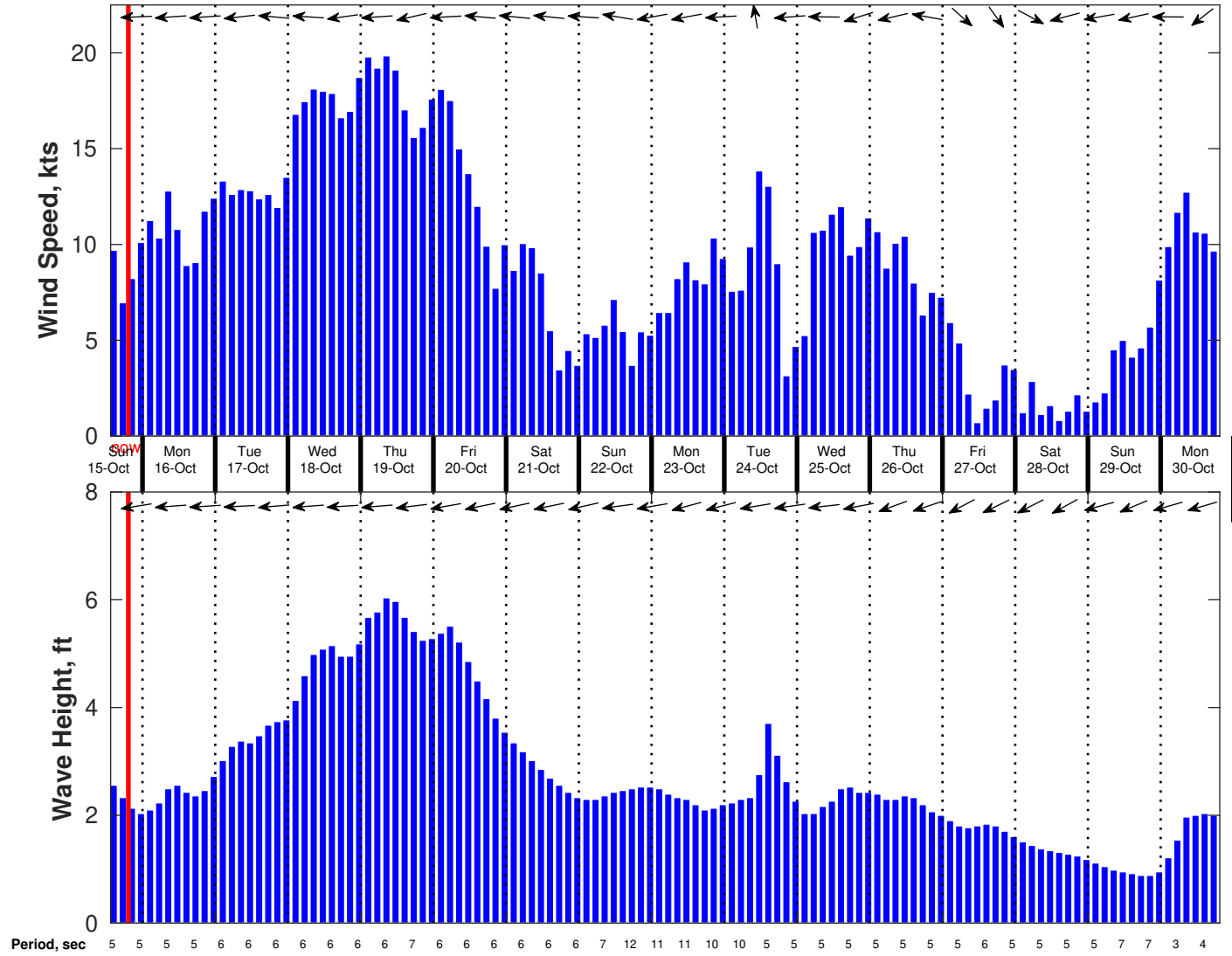
Wind & Wave Forecast for OXY Colombia Geotech Col6 from 15-Oct-2023 13:00:00 to 31-Oct-2023 13:00:00
