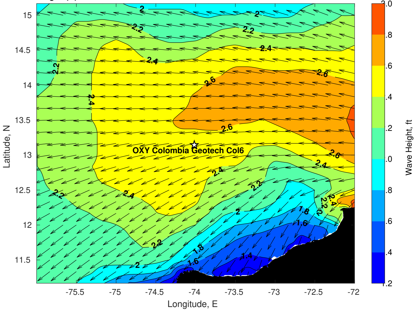
Wave Height (ft) for OXY Colombia Geotech Col6 at 15-Oct-2023 18:00:00
