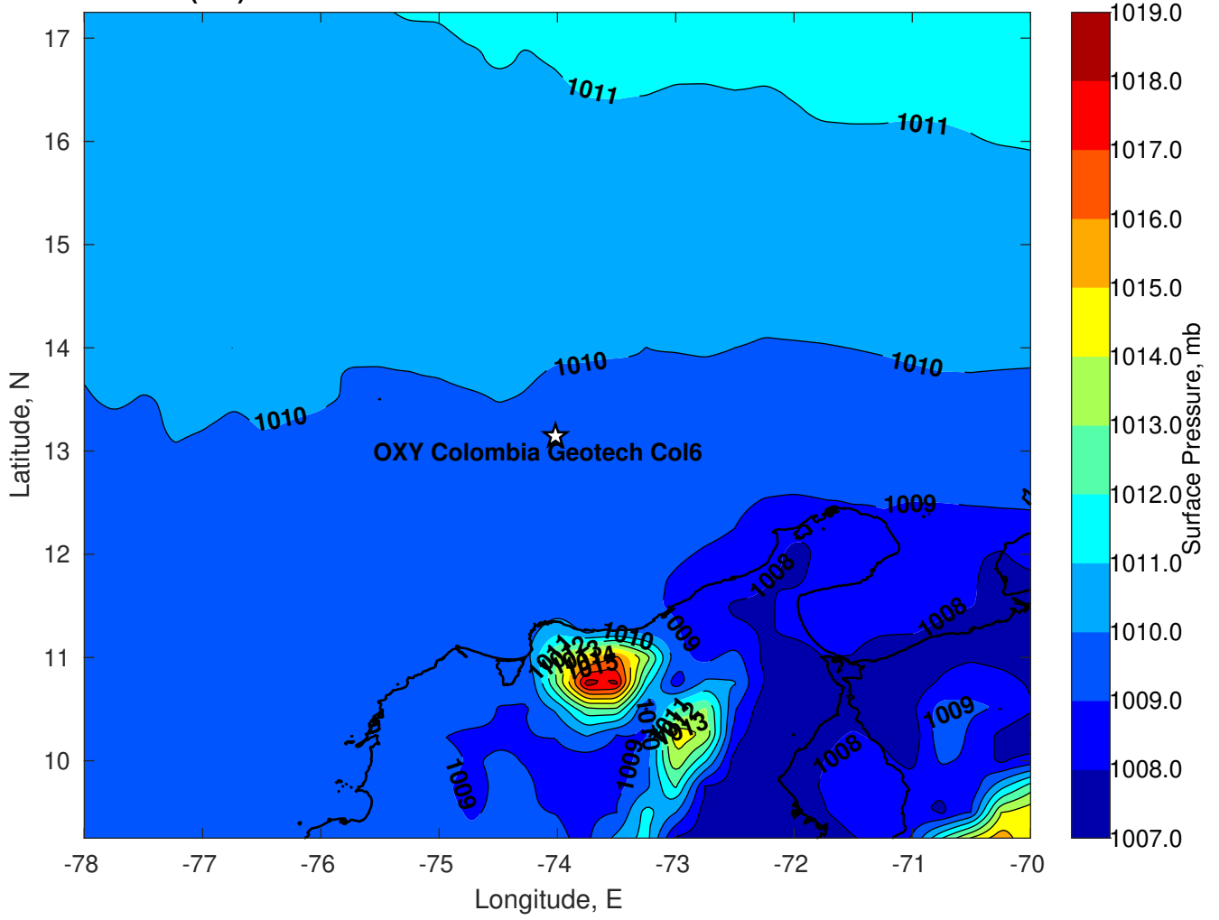
Surface Pressure (mb) for OXY Colombia Geotech Col6 at 16-Oct-2023 18:00:00
