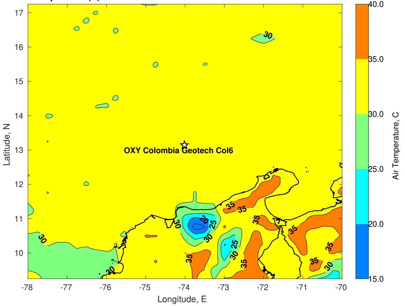
Air Temperature (C) for OXY Colombia Geotech Col6 at 15-Oct-2023
