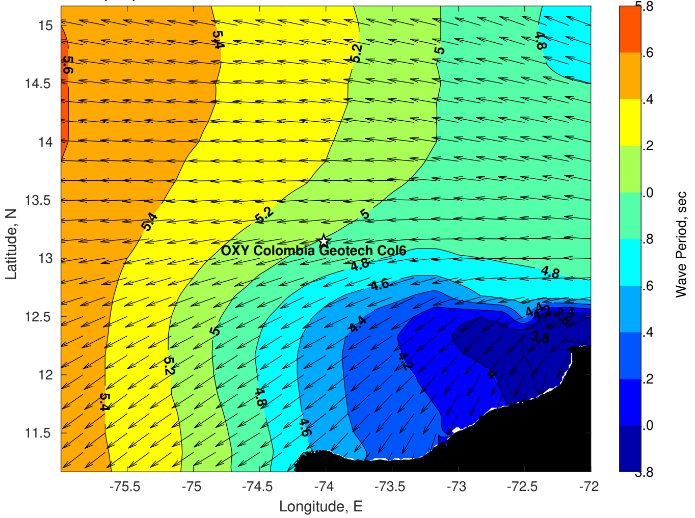
Wave Period (sec) for OXY Colombia Geotech Col6 at 15-Oct-2023 18:00:00
