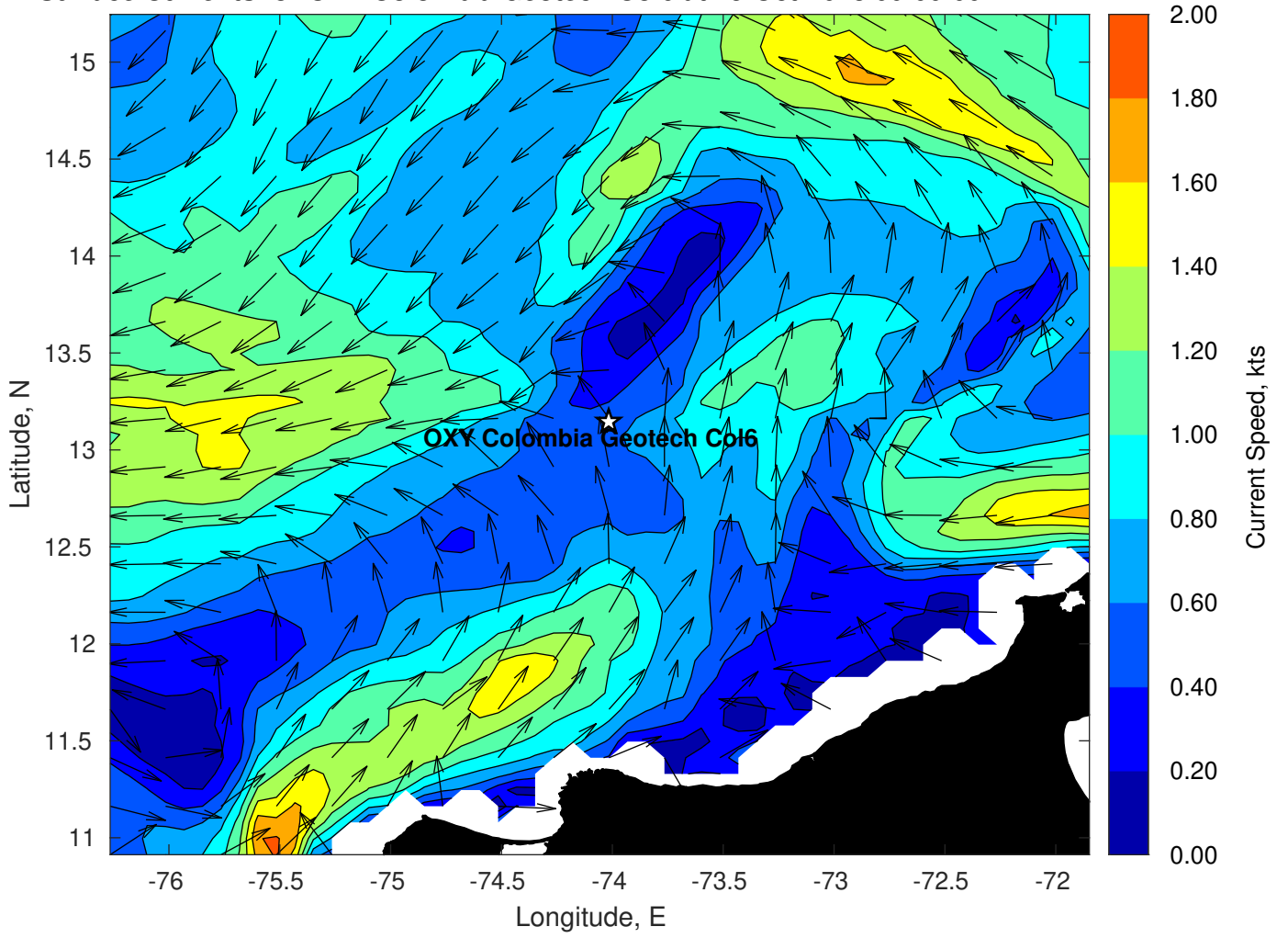
Surface Currents for OXY Colombia Geotech Col6 at 15-Oct-2023 00:00:00
