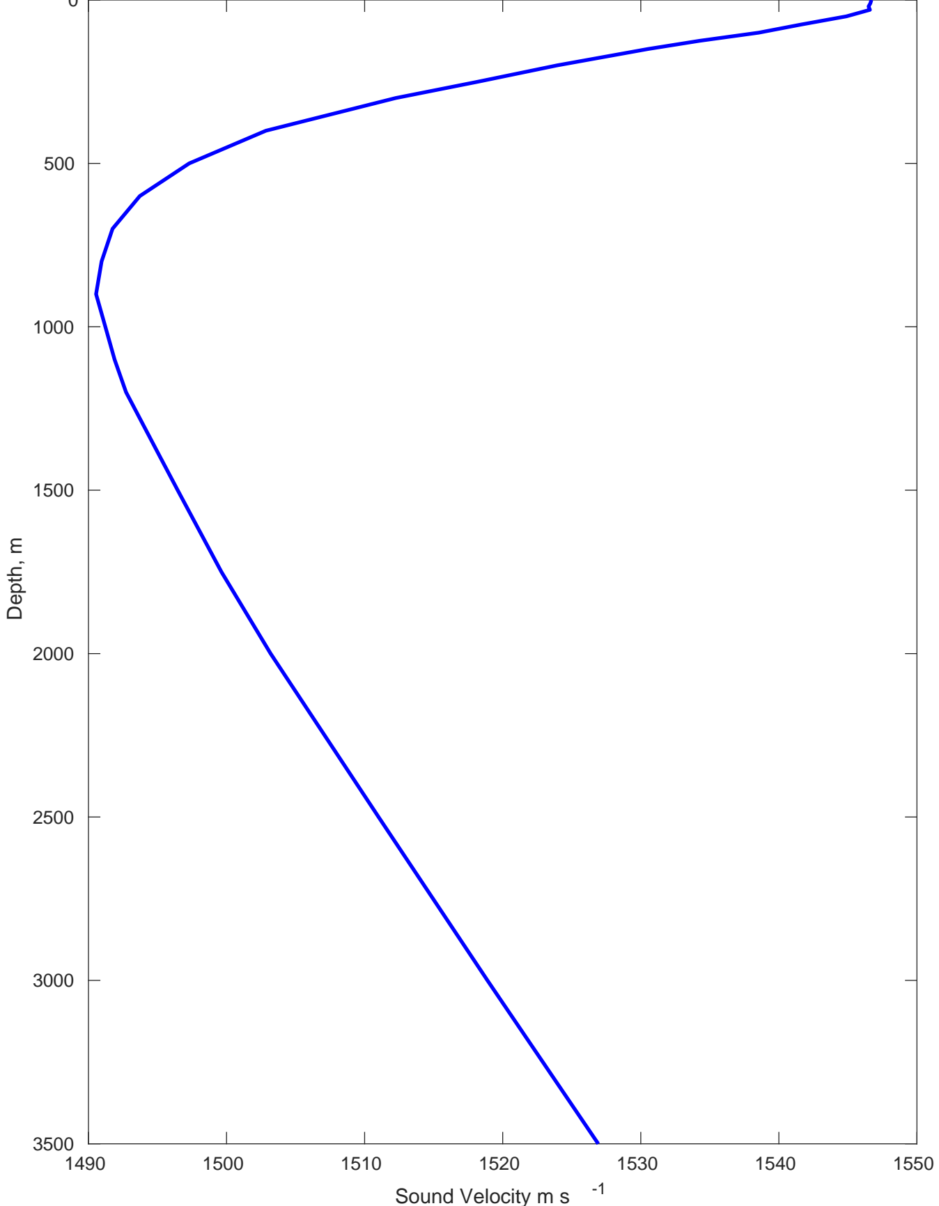
Sound Velocity Profile for OXY Colombia Geotech Col6 on 15-Oct-2023 00:00:00
