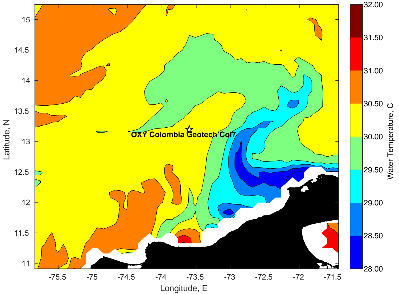
SST for OXY Colombia Geotech Col7 at 15-Oct-2023 00:00:00
