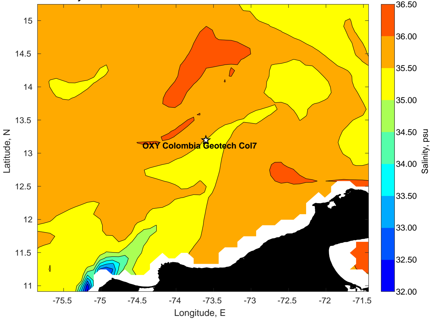
Surface Salinity for OXY Colombia Geotech Col7 at 15-Oct-2023 00:00:00
