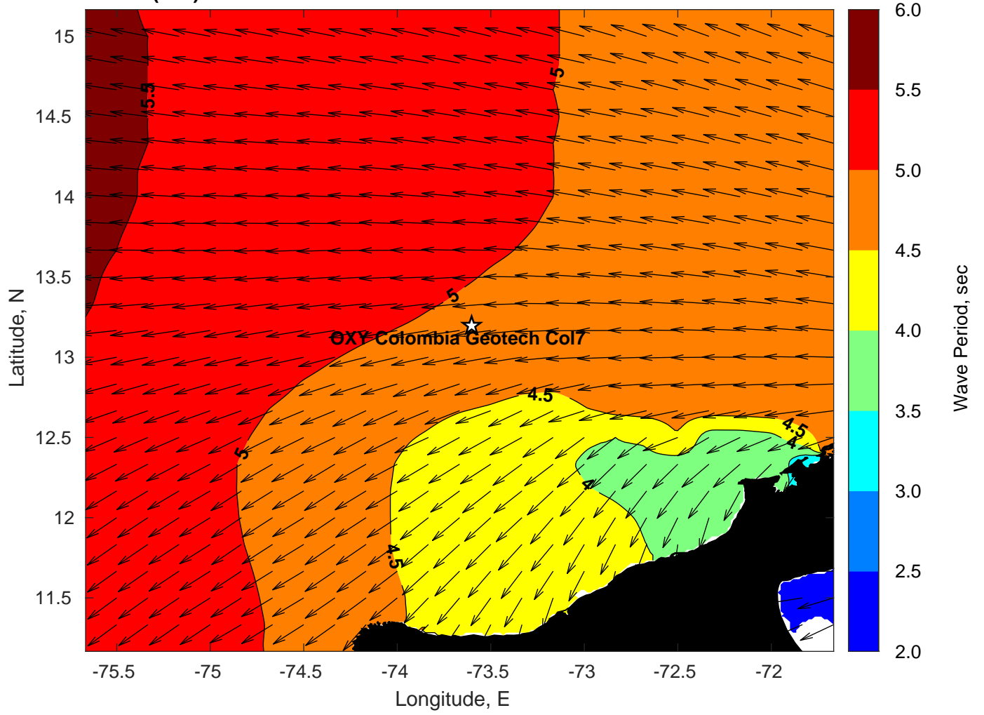
Wave Period (sec) for OXY Colombia Geotech Col7 at 15-Oct-2023 18:00:00
