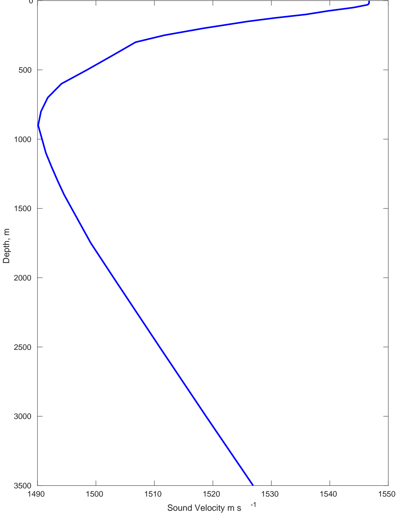
Sound Velocity Profile for OXY Colombia Geotech Col7 on 15-Oct-2023 00:00:00
