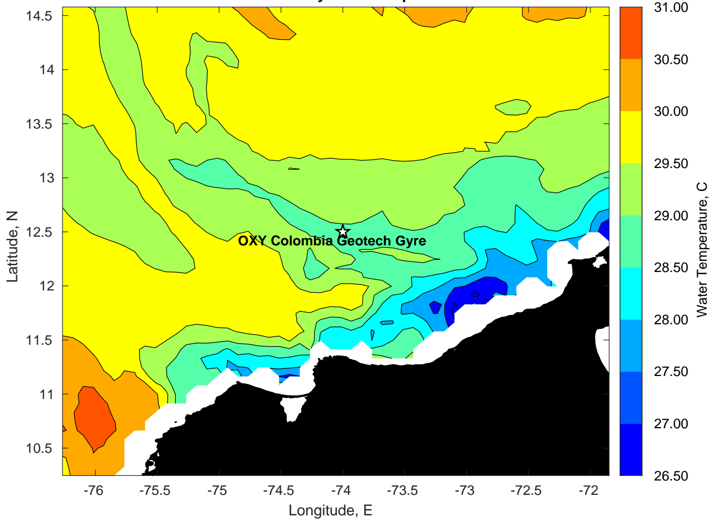
SST for OXY Colombia Geotech Gyre at 18-Sep-2023 00:00:00
