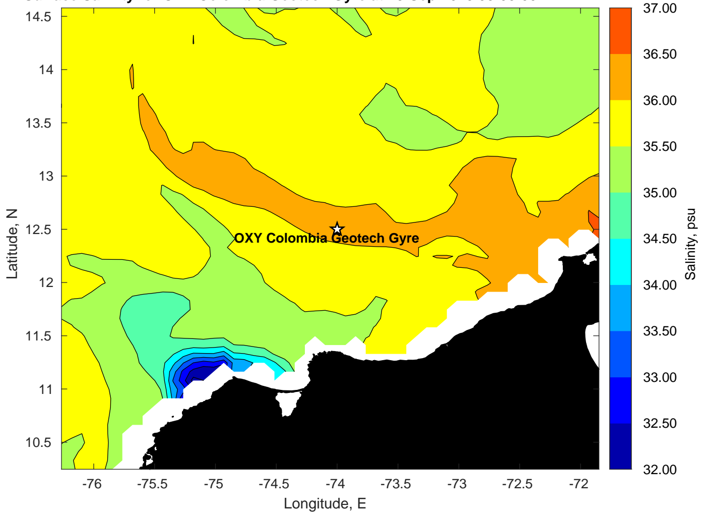
Surface Salinity for OXY Colombia Geotech Gyre at 18-Sep-2023 00:00:00
