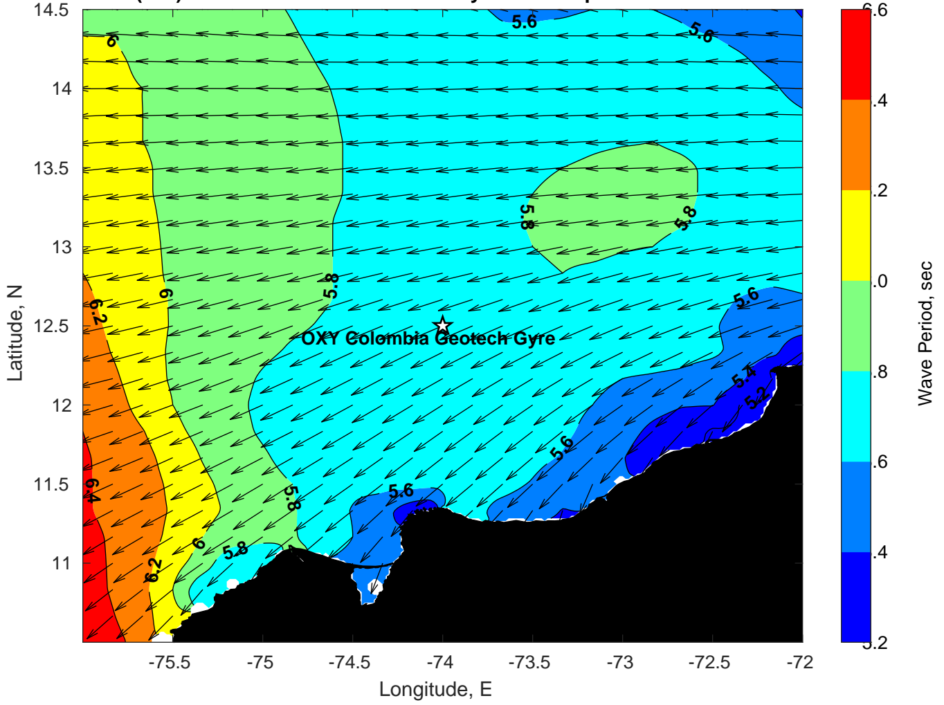
Wave Period (sec) for OXY Colombia Geotech Gyre at 18-Sep-2023 18:00:00
