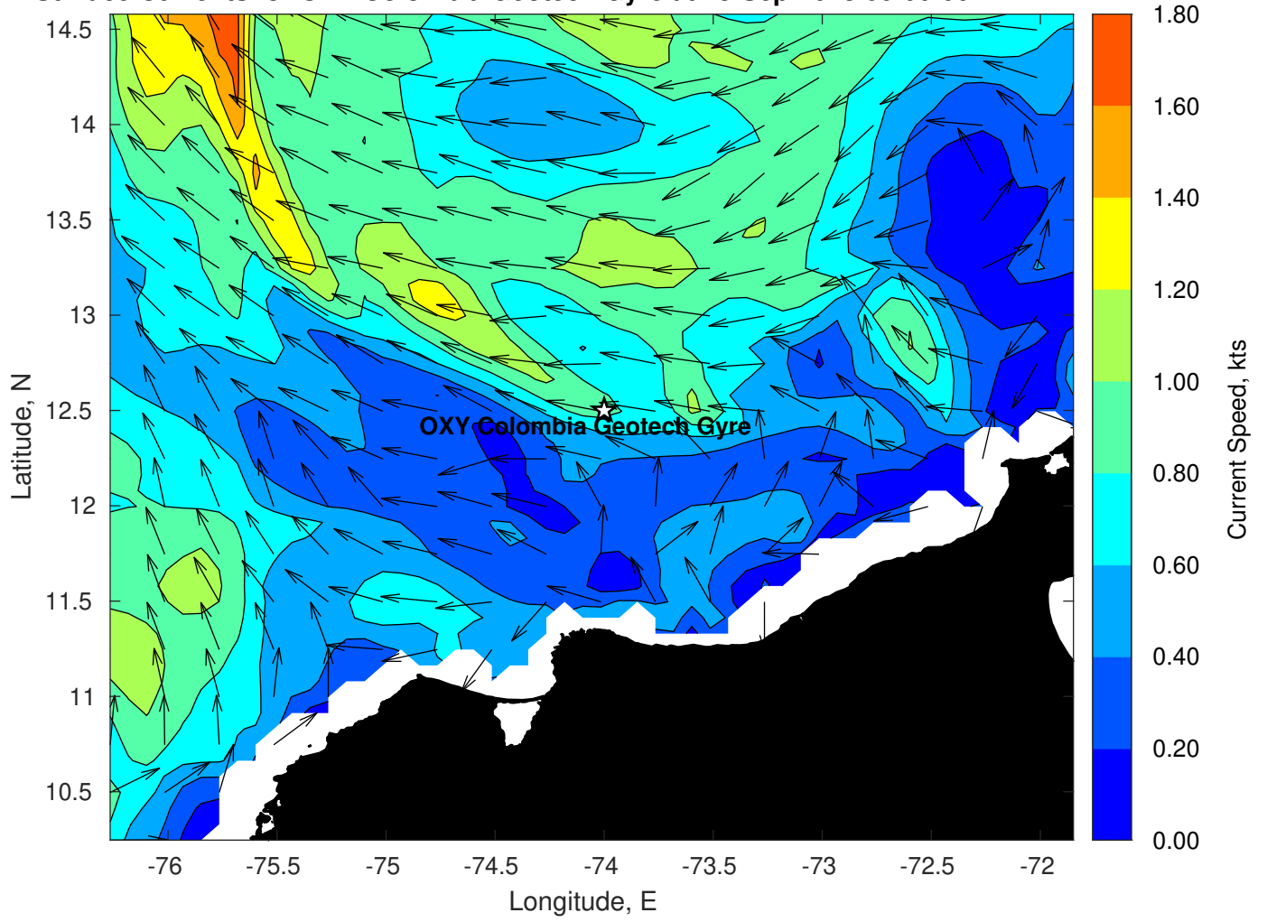
Surface Currents for OXY Colombia Geotech Gyre at 18-Sep-2023 00:00:00
