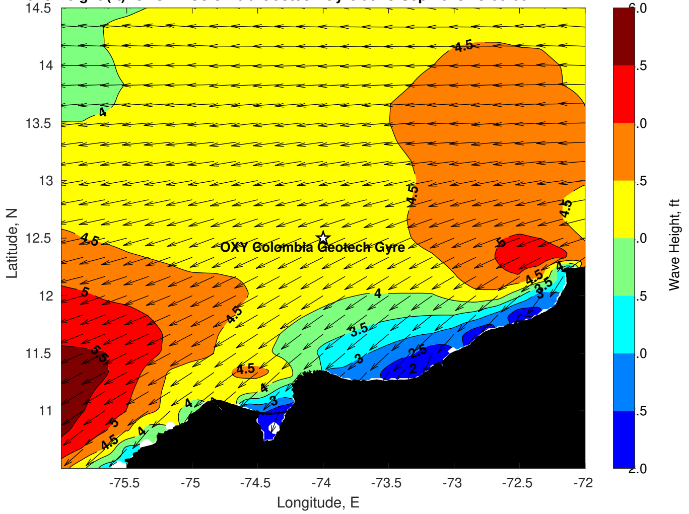
Wave Height (ft) for OXY Colombia Geotech Gyre at 18-Sep-2023 18:00:00
