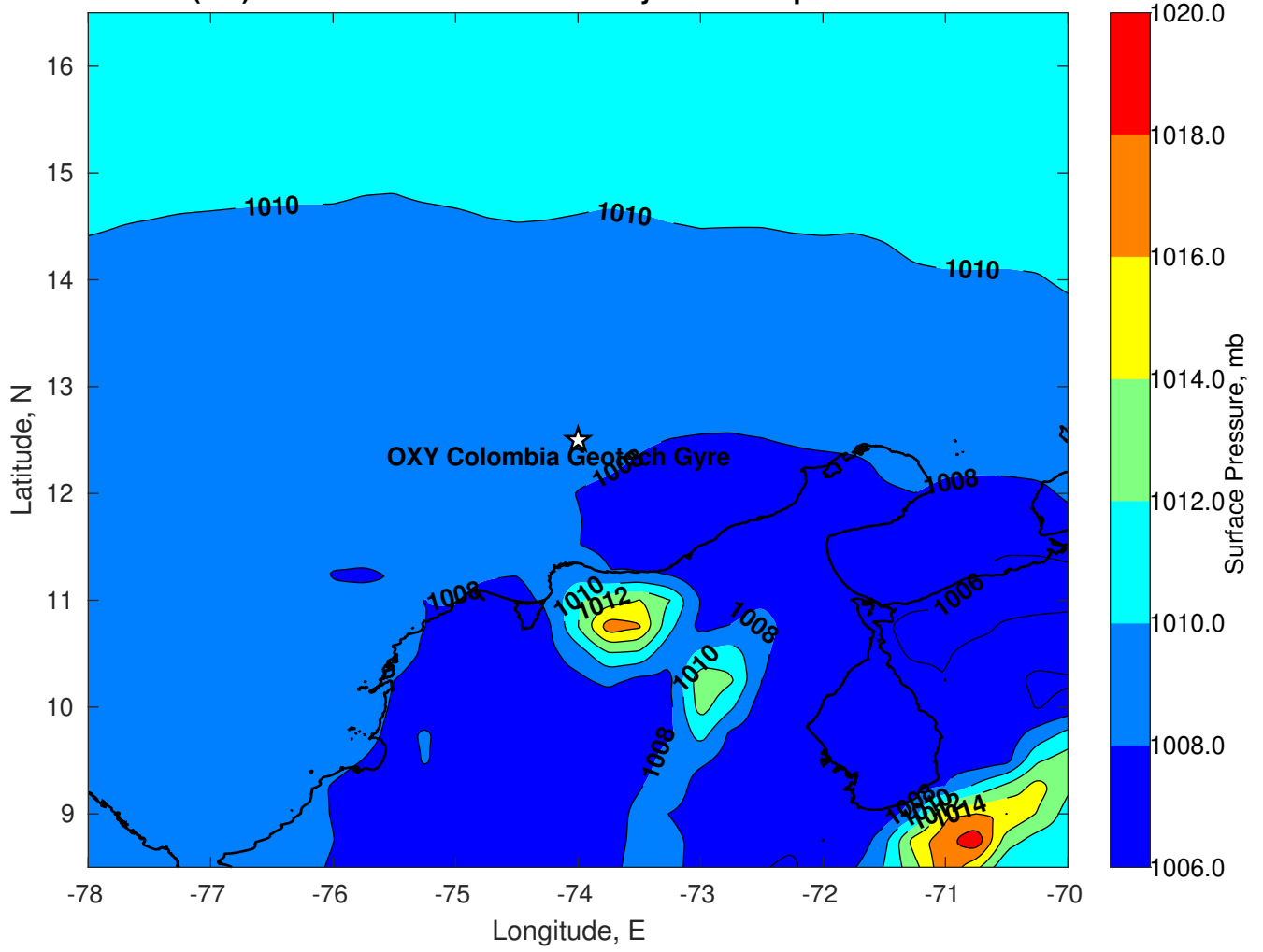
Surface Pressure (mb) for OXY Colombia Geotech Gyre at 20-Sep-2023 18:00:00
