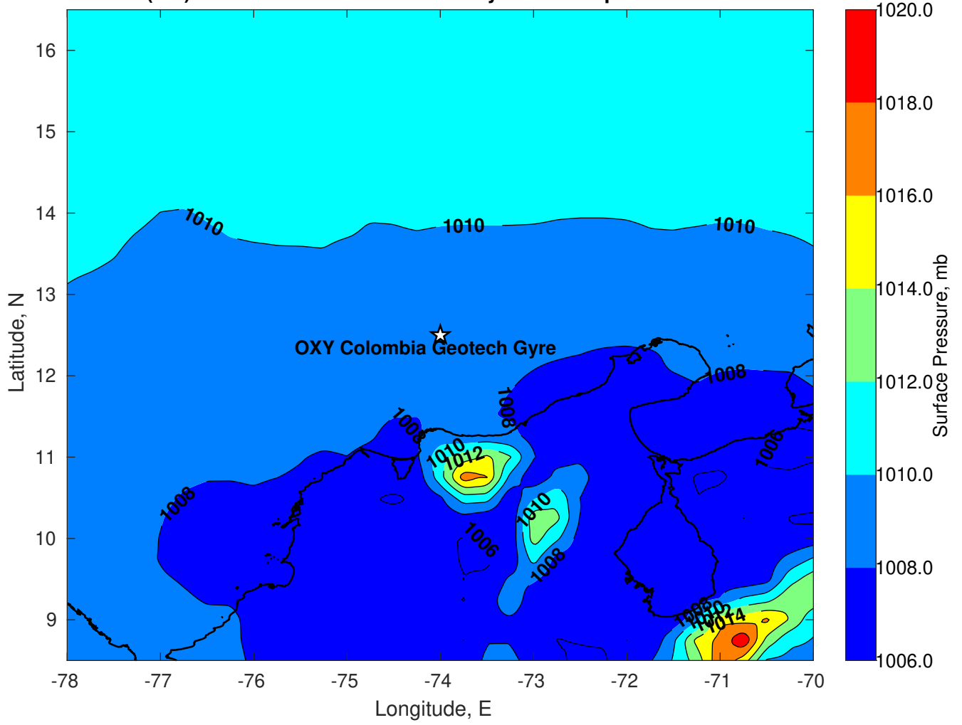
Surface Pressure (mb) for OXY Colombia Geotech Gyre at 18-Sep-2023 18:00:00
