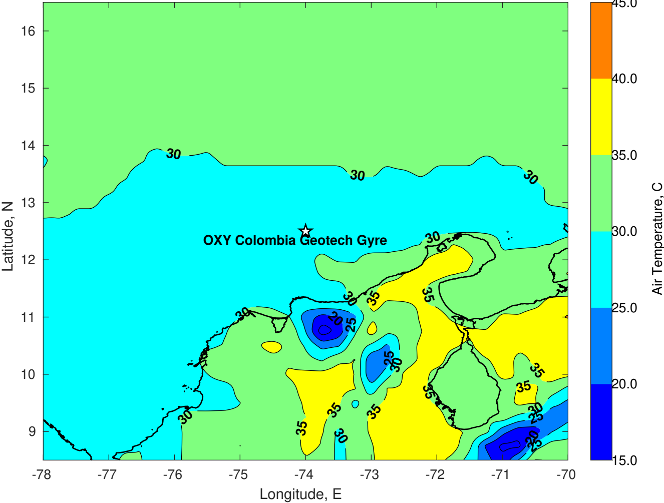
Air Temperature (C) for OXY Colombia Geotech Gyre at 18-Sep-2023
