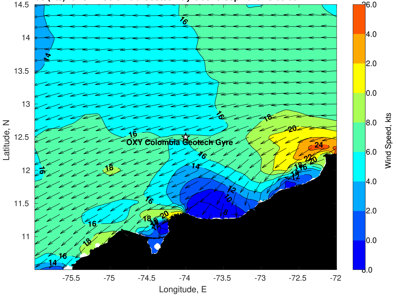
Winds (kts) for OXY Colombia Geotech Gyre at 18-Sep-2023 18:00:00
