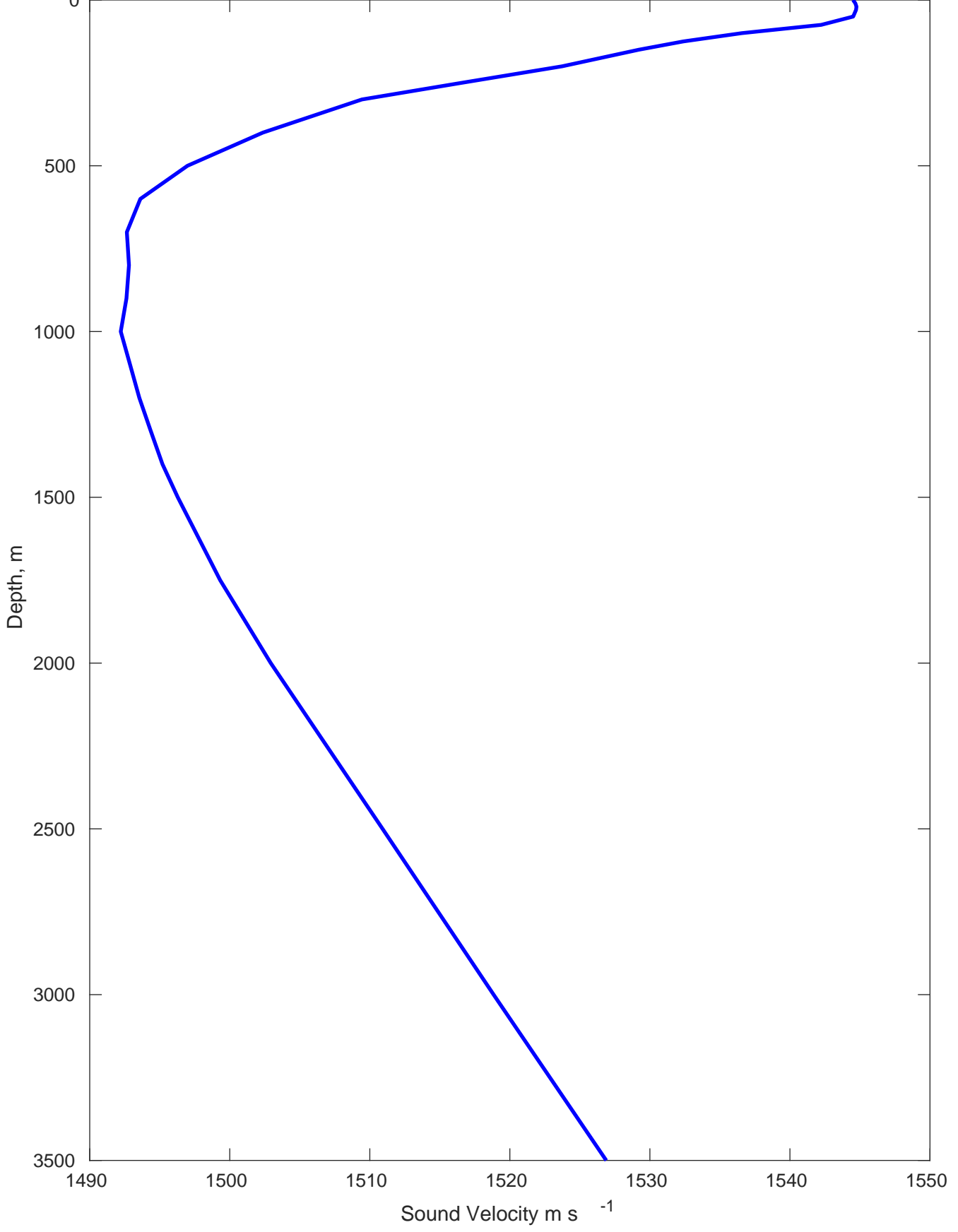
Sound Velocity Profile for OXY Colombia Geotech Gyre on 18-Sep-2023 00:00:00
