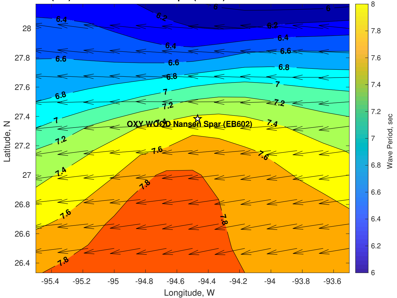
Wave Period (sec) for OXY WOOD Nansen Spar (EB602) at 18-Oct-2024 06:00:00
