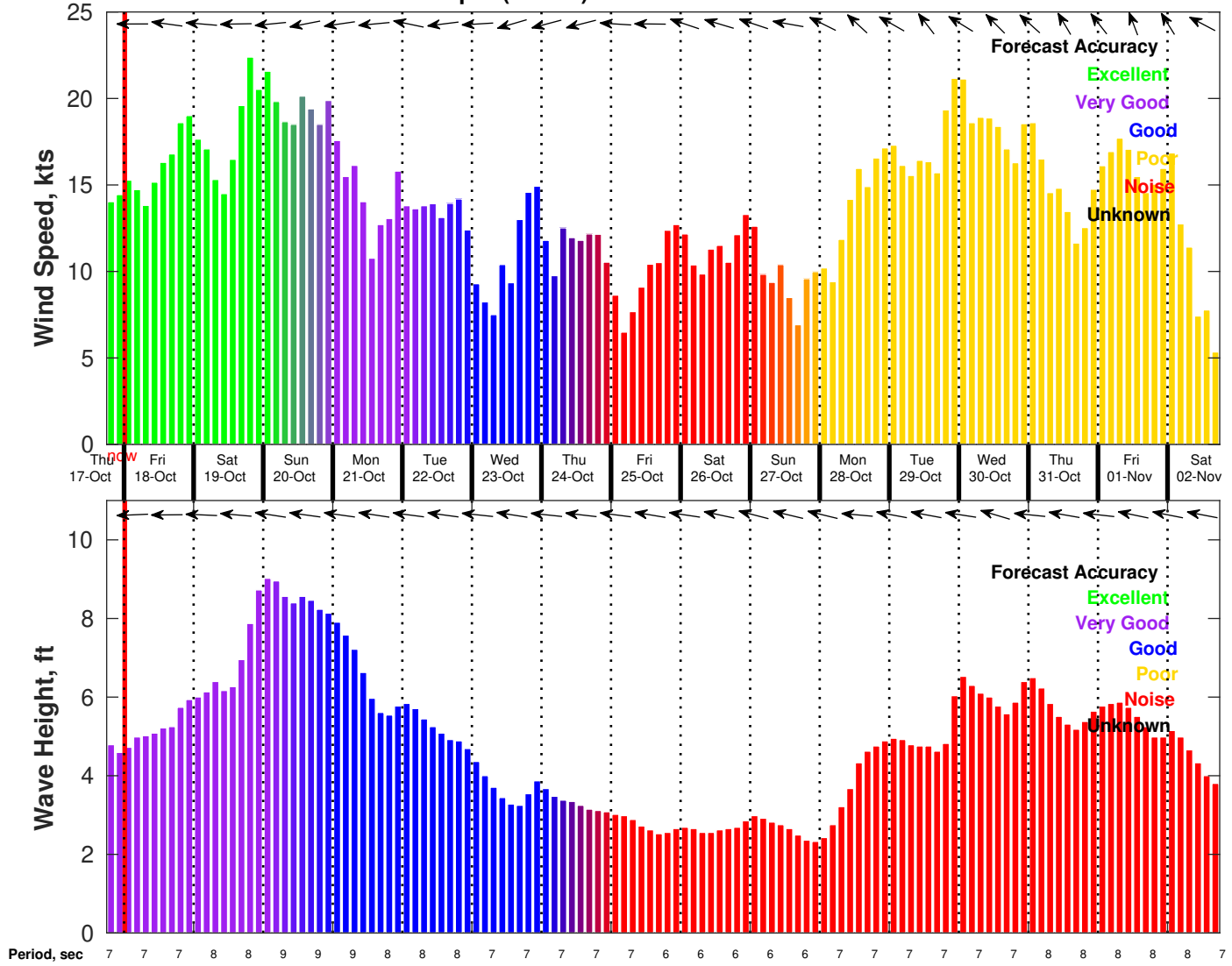
Wind & Wave Forecast for OXY WOOD Nansen Spar (EB602) from 17-Oct-2024 18:00:00 to 02-Nov-2024 18:00:00
