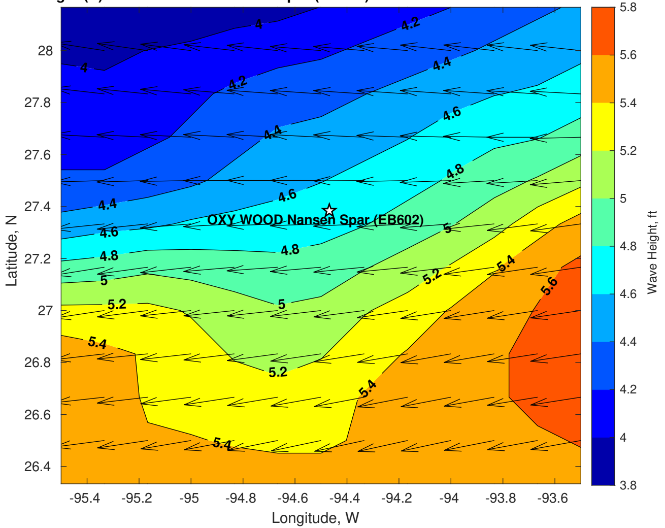
Wave Height (ft) for OXY WOOD Nansen Spar (EB602) at 18-Oct-2024 06:00:00
