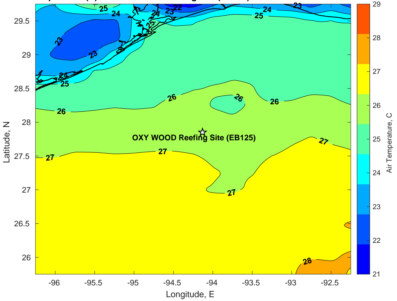
Air Temperature (C) for OXY WOOD Reefing Site (EB125) at 18-Oct-2024
