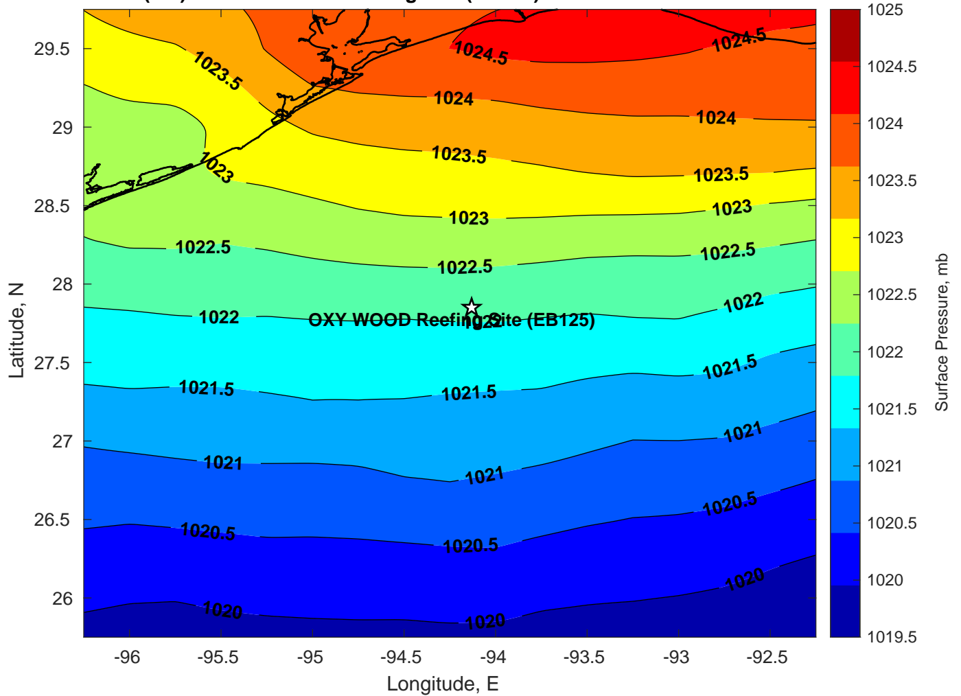
Surface Pressure (mb) for OXY WOOD Reefing Site (EB125) at 17-Oct-2024 18:00:00
