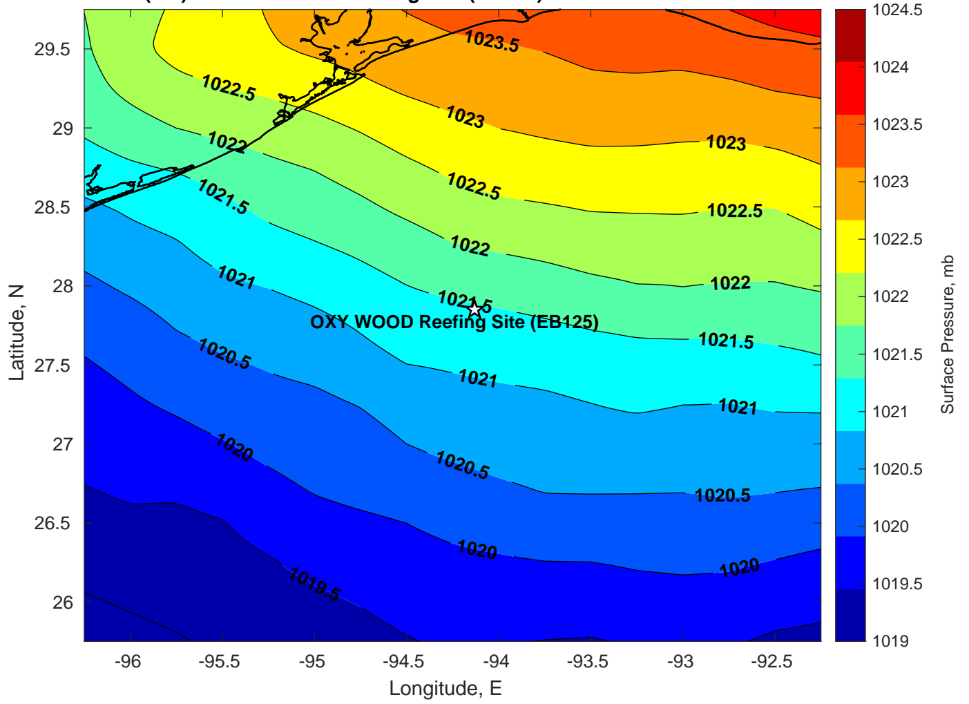
Surface Pressure (mb) for OXY WOOD Reefing Site (EB125) at 19-Oct-2024 00:00:00
