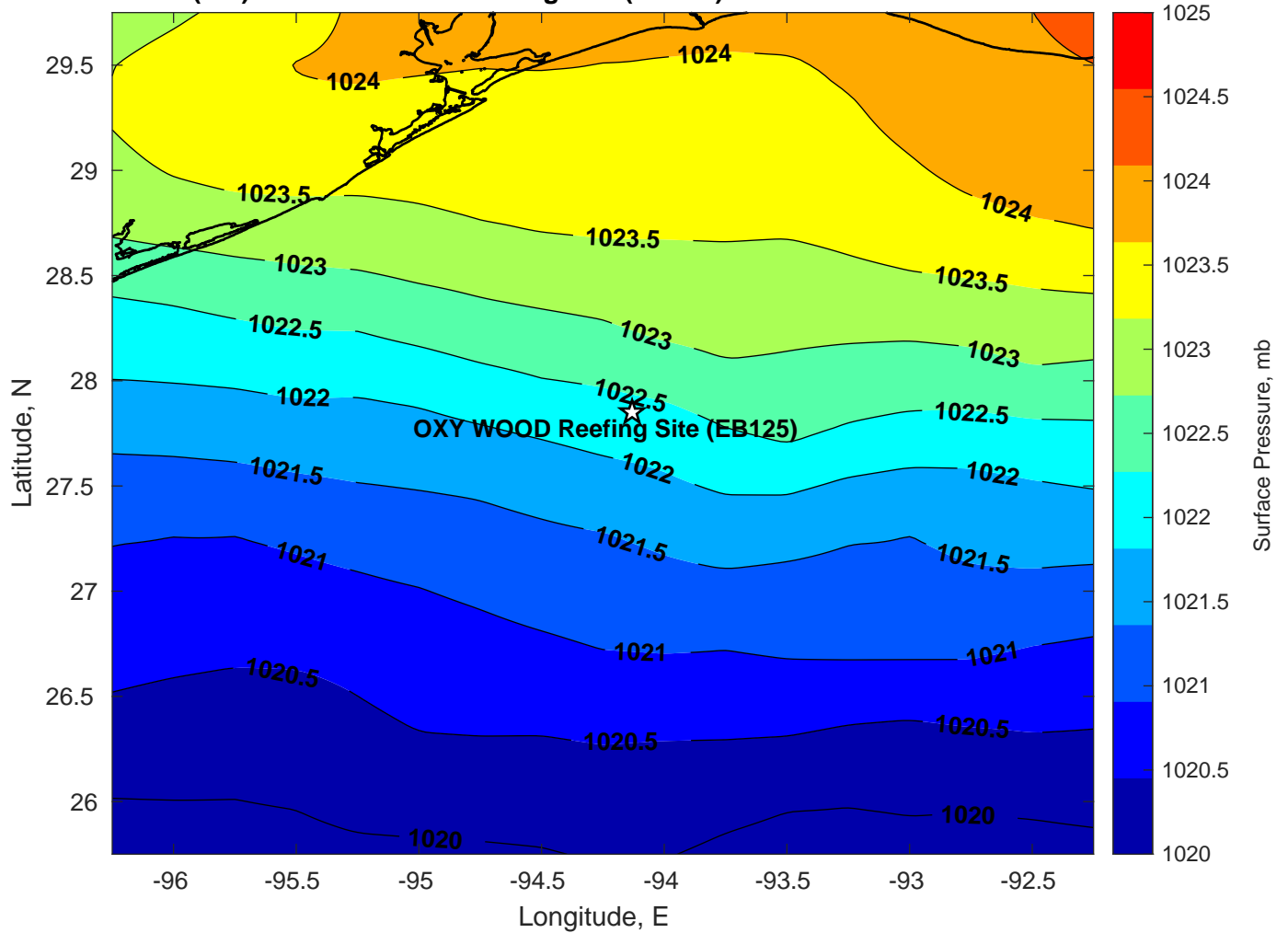
Surface Pressure (mb) for OXY WOOD Reefing Site (EB125) at 20-Oct-2024 00:00:00
