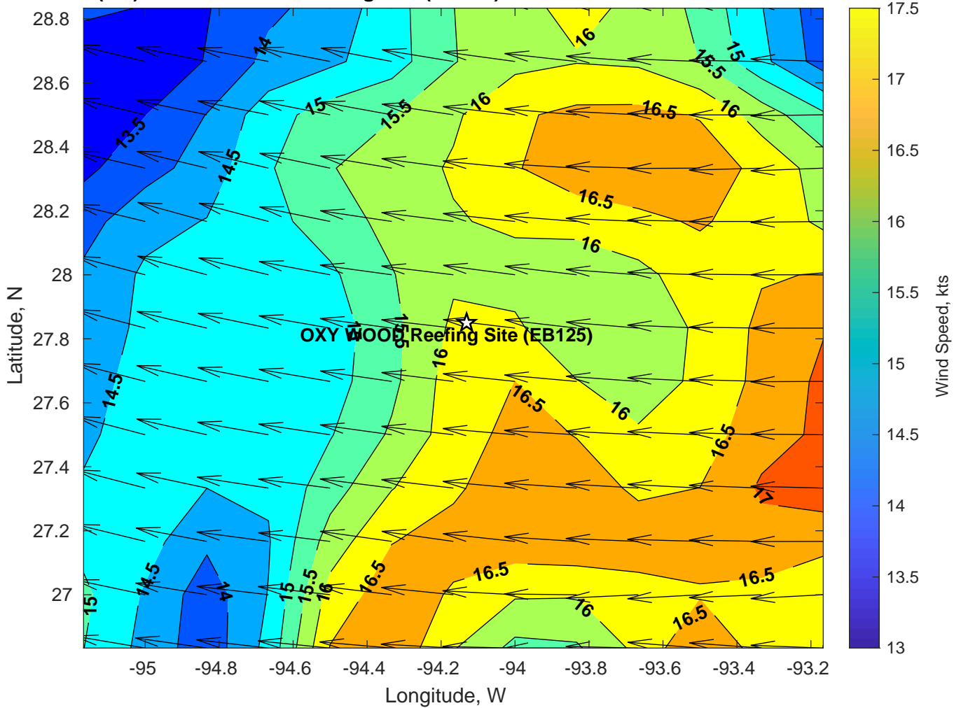
Winds (kts) for OXY WOOD Reefing Site (EB125) at 18-Oct-2024 06:00:00
