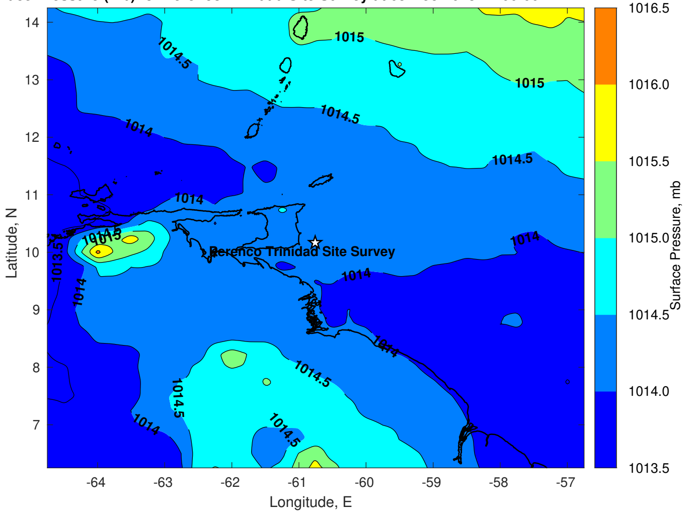
Surface Pressure (mb) for Perenco Trinidad Site Survey at 05-Dec-2023 12:00:00
