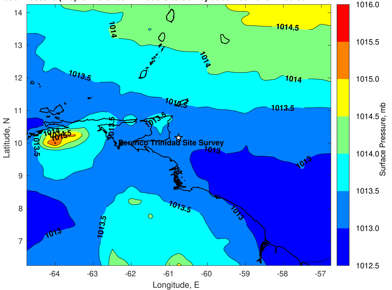
Surface Pressure (mb) for Perenco Trinidad Site Survey at 03-Dec-2023 12:00:00
