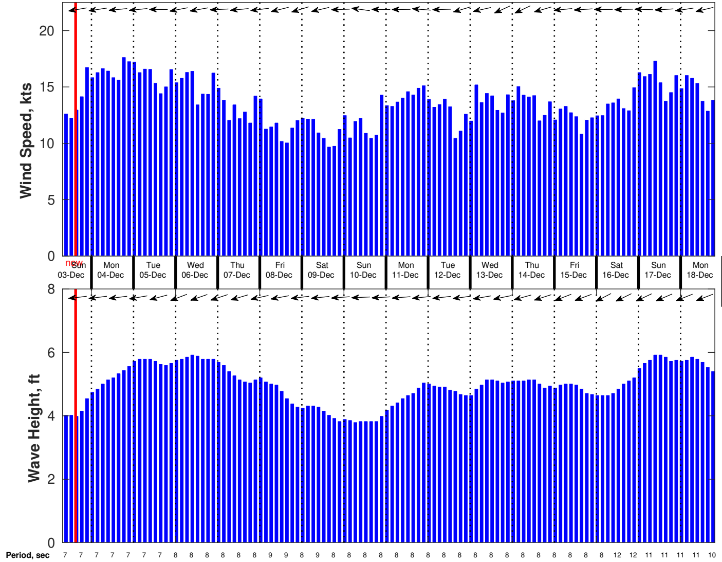
Wind & Wave Forecast for Perenco Trinidad Site Survey from 03-Dec-2023 08:00:00 to 19-Dec-2023 08:00:00
