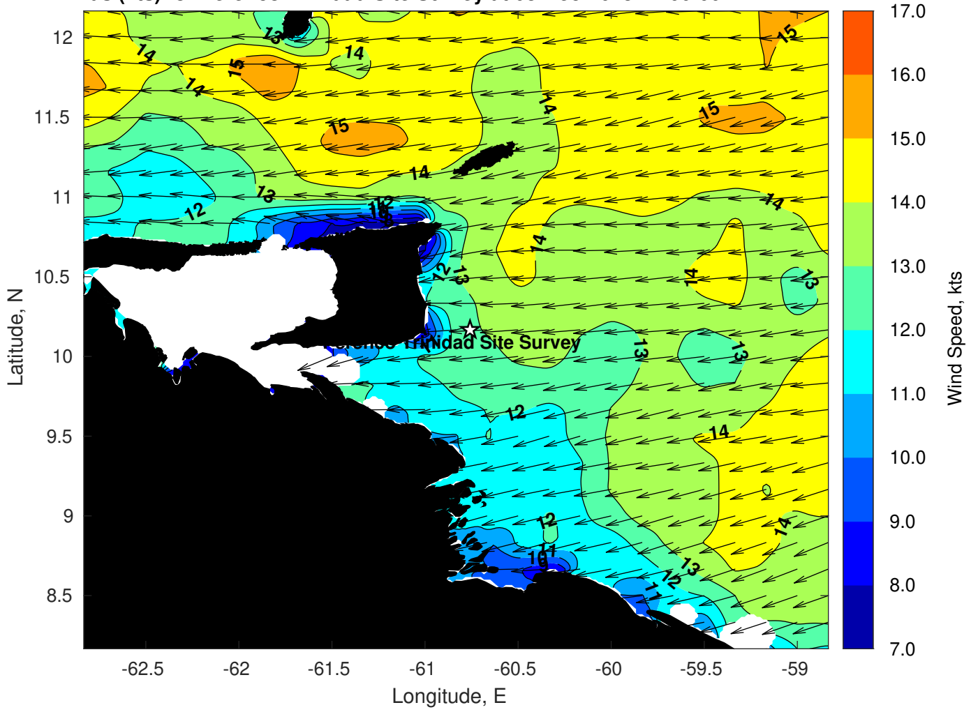
Winds (kts) for Perenco Trinidad Site Survey at 03-Dec-2023 12:00:00
