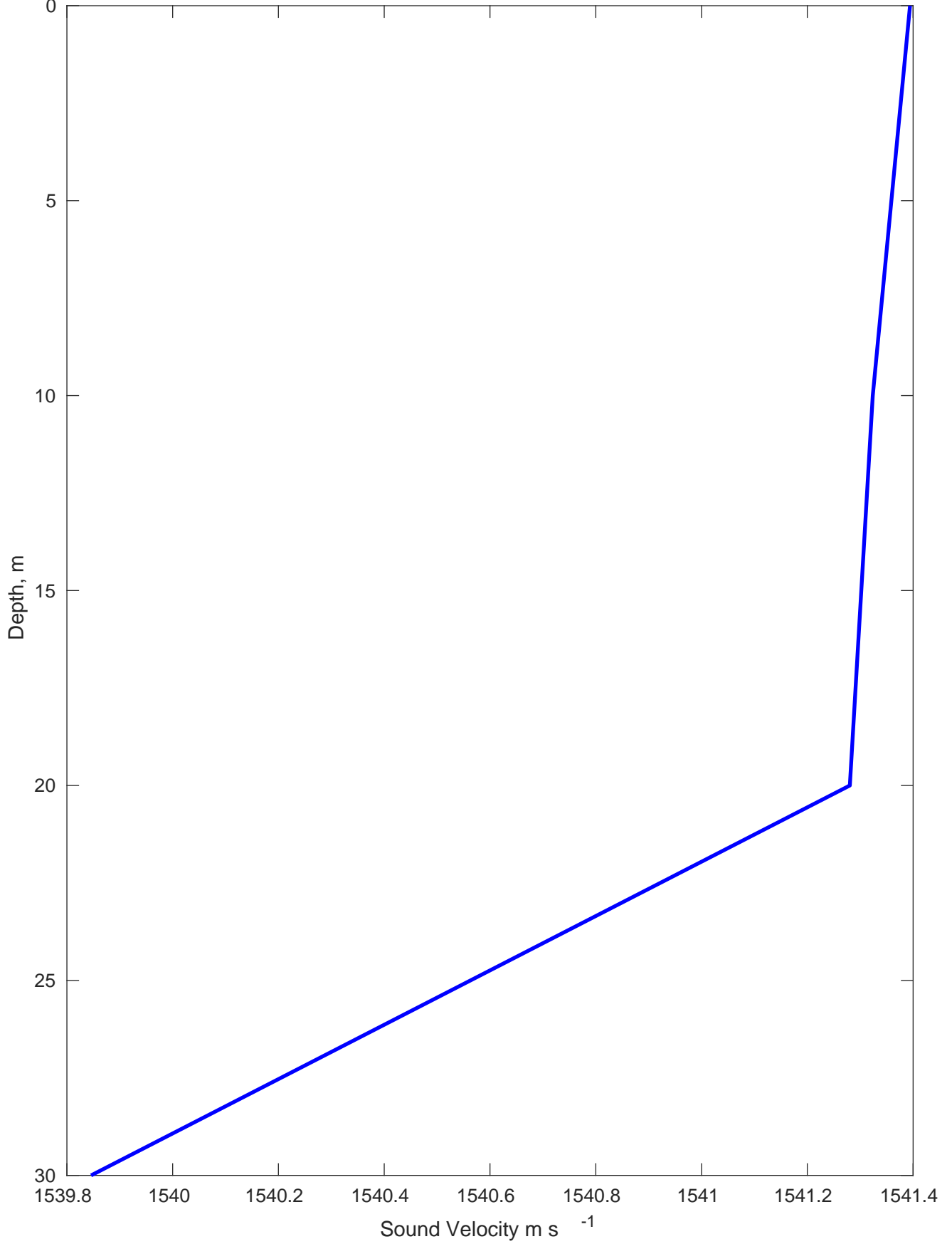
Sound Velocity Profile for Perenco Trinidad Site Survey on 03-Dec-2023 00:00:00
