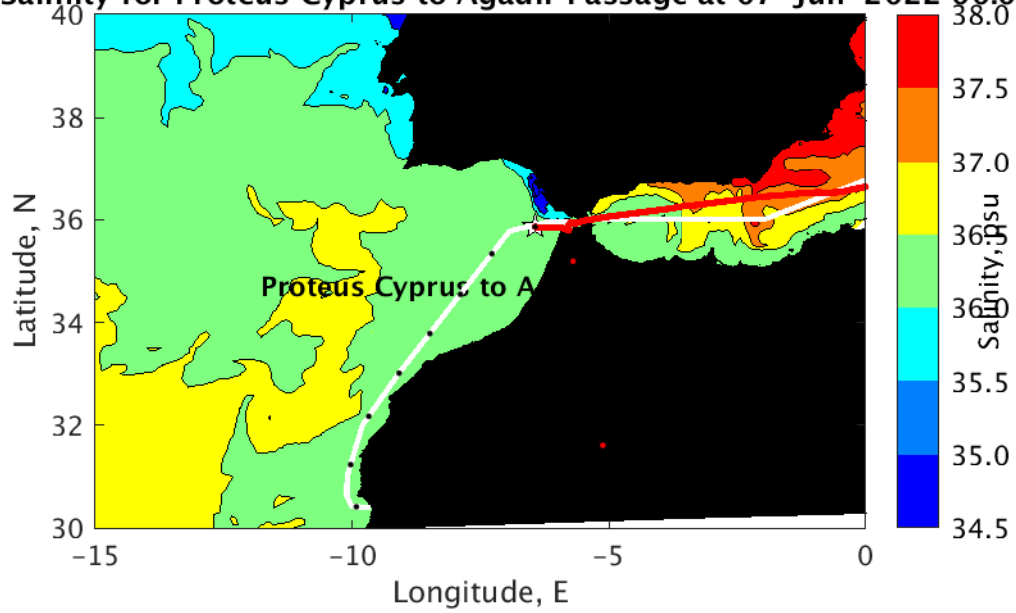
Sea Salinity for Proteus Cyprus to Agadir Passage at 07-Jun-2022 00:00:00
