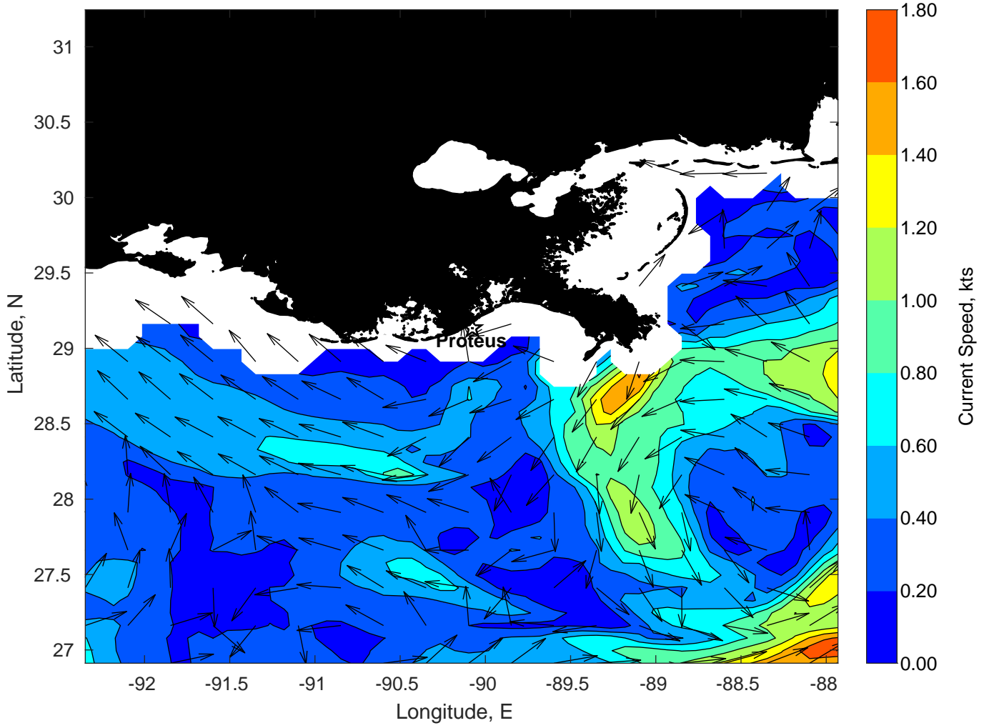
Surface Currents for Proteus at 08-Feb-2023 00:00:00
