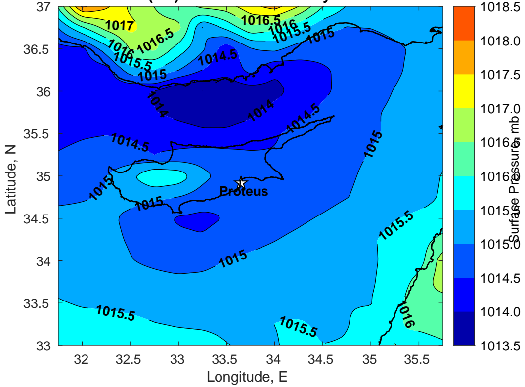
Surface Pressure (mb) for Proteus at 17-May-2022 00:00:00
