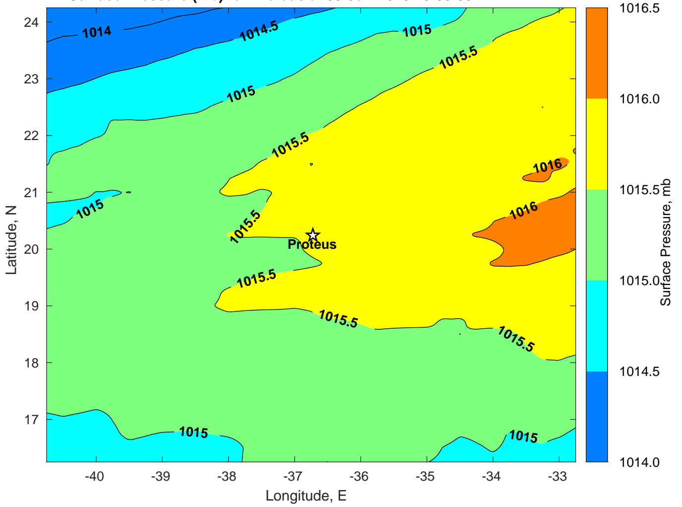
Surface Pressure (mb) for Proteus at 03-Jun-2023 18:00:00
