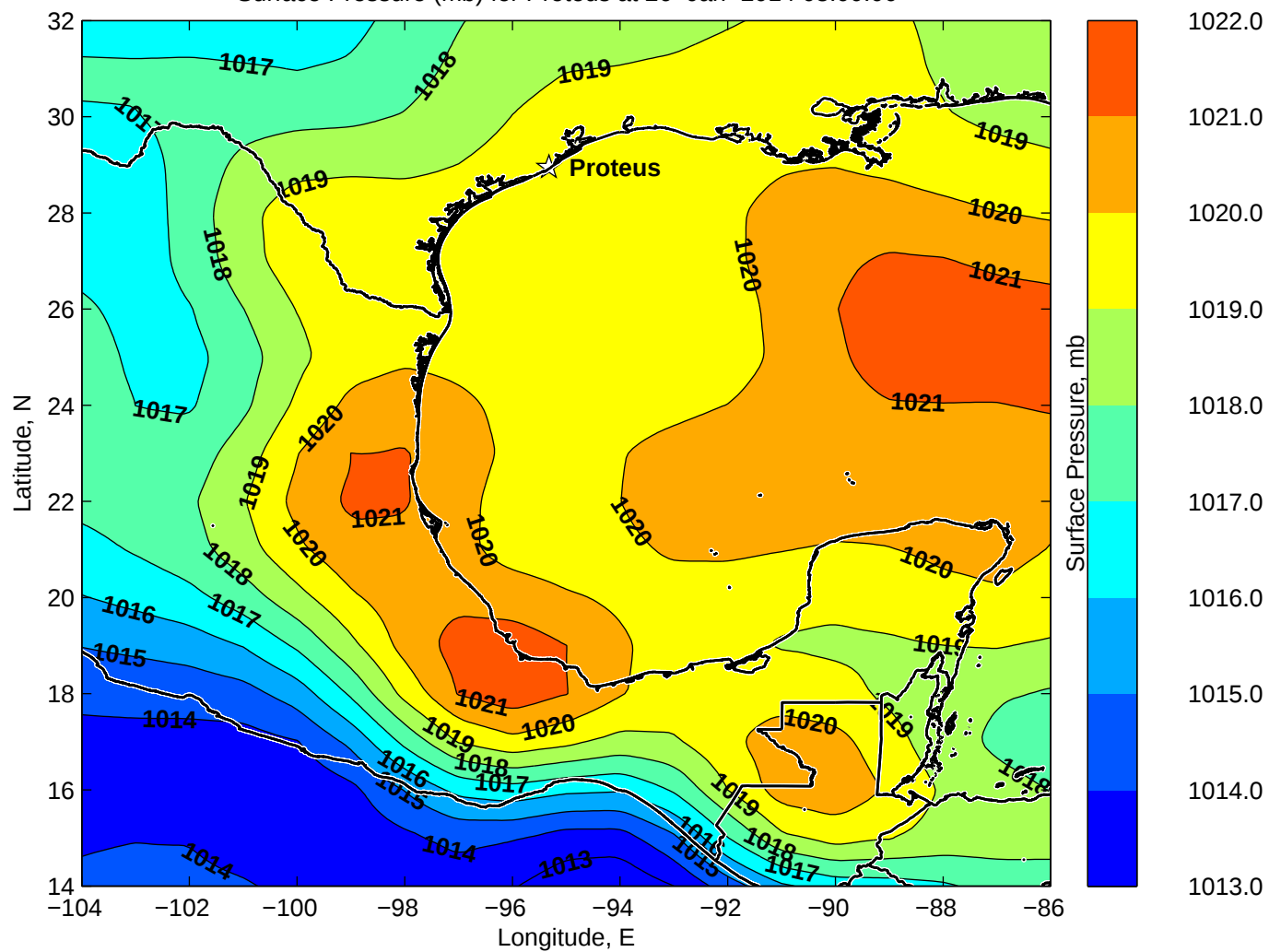
Surface Pressure (mb) for Proteus at 26-Jan-2014 03:00:00
