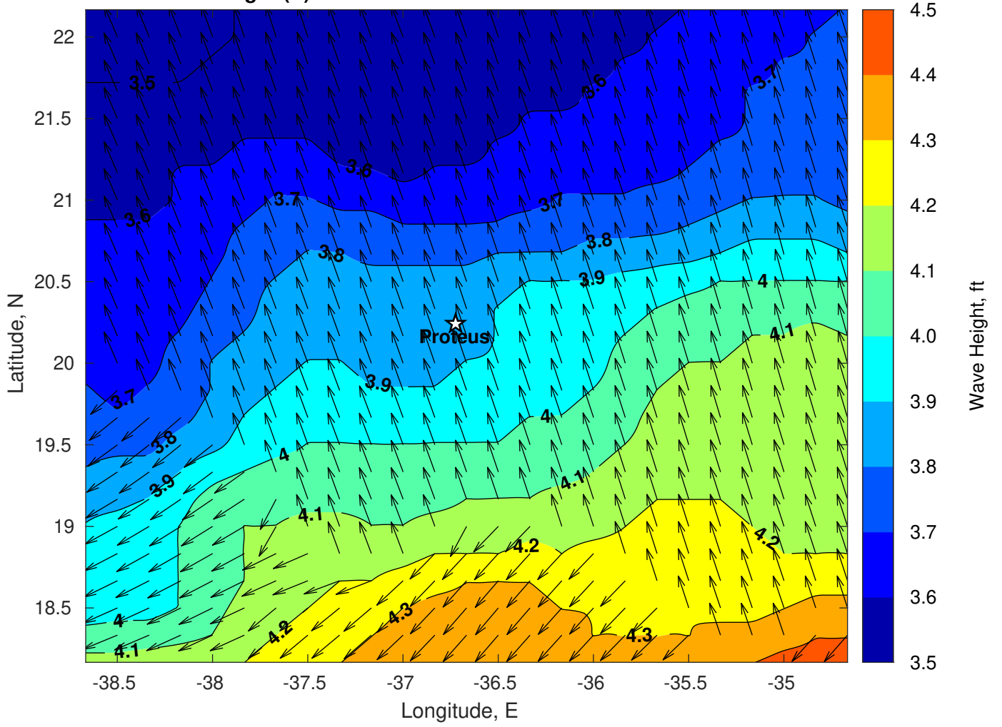
Wave Height (ft) for Proteus at 01-Jun-2023 18:00:00
