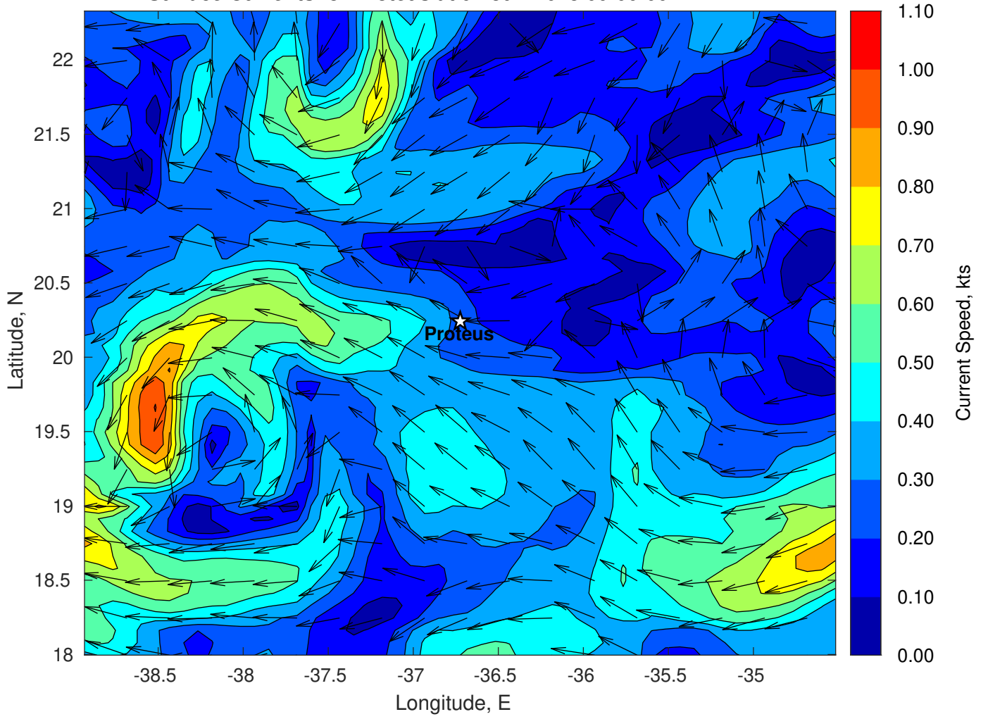
Surface Currents for Proteus at 01-Jun-2023 00:00:00
