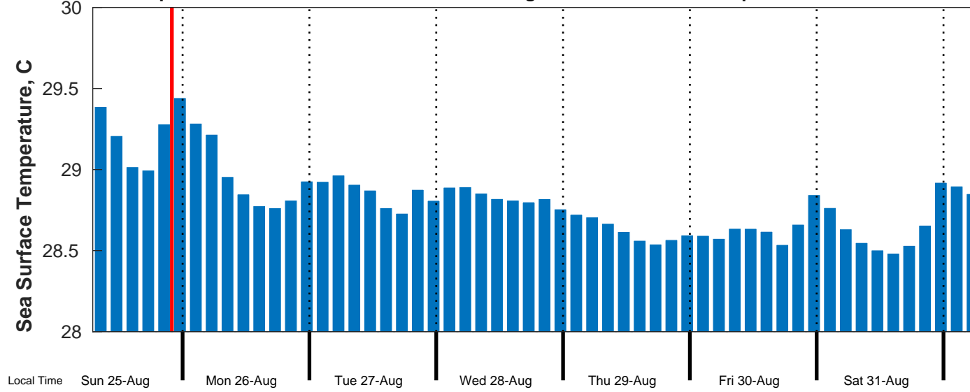
Sea Surface Temperature Forecast for Proteus from 26-Aug-2024 00:00:00 to 02-Sep-2024 00:00:00
