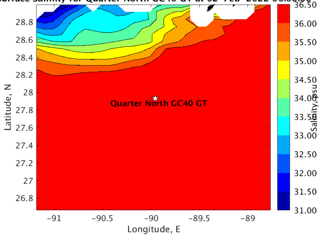
Surface Salinity for Quarter North GC40 GT at 02-Feb-2022 00:00:00
