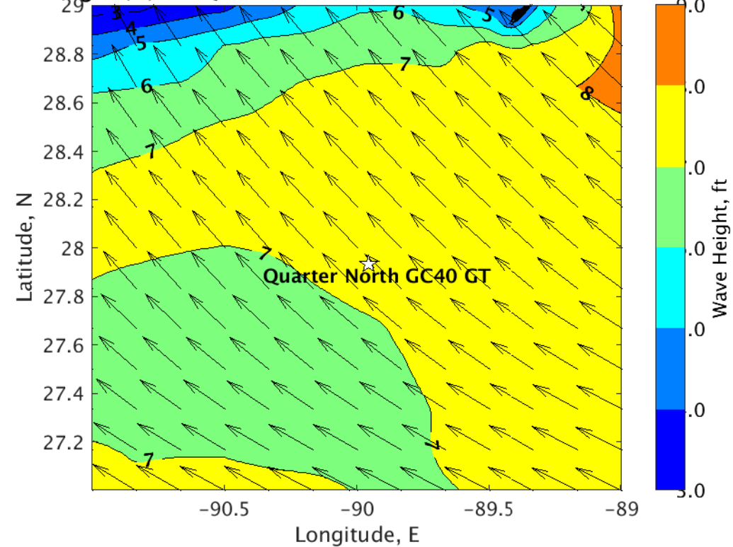
ave Height (ft) for Quarter North GC40 GT at 02-Feb-2022 12:00:00
