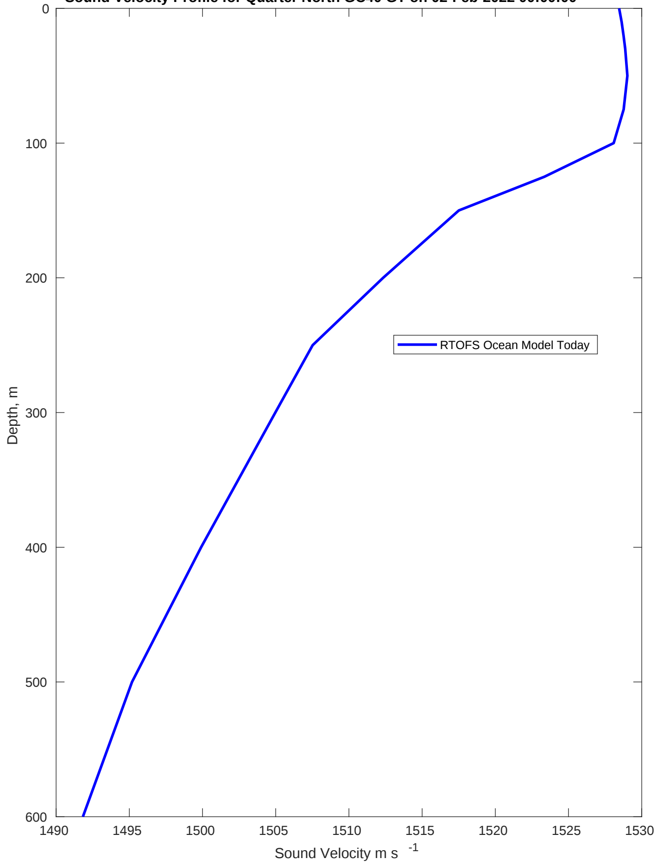
Sound Velocity Profile for Quarter North GC40 GT on 02-Feb-2022 00:00:00
