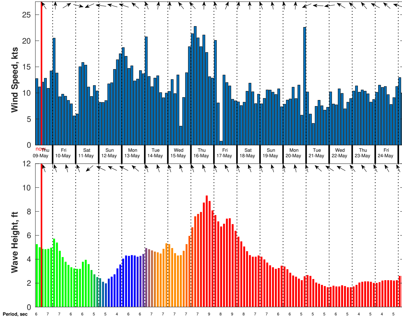
Wind & Wave Forecast for Shell Zephyrus GT from 09-May-2024 06:00:00 to 25-May-2024 06:00:00
