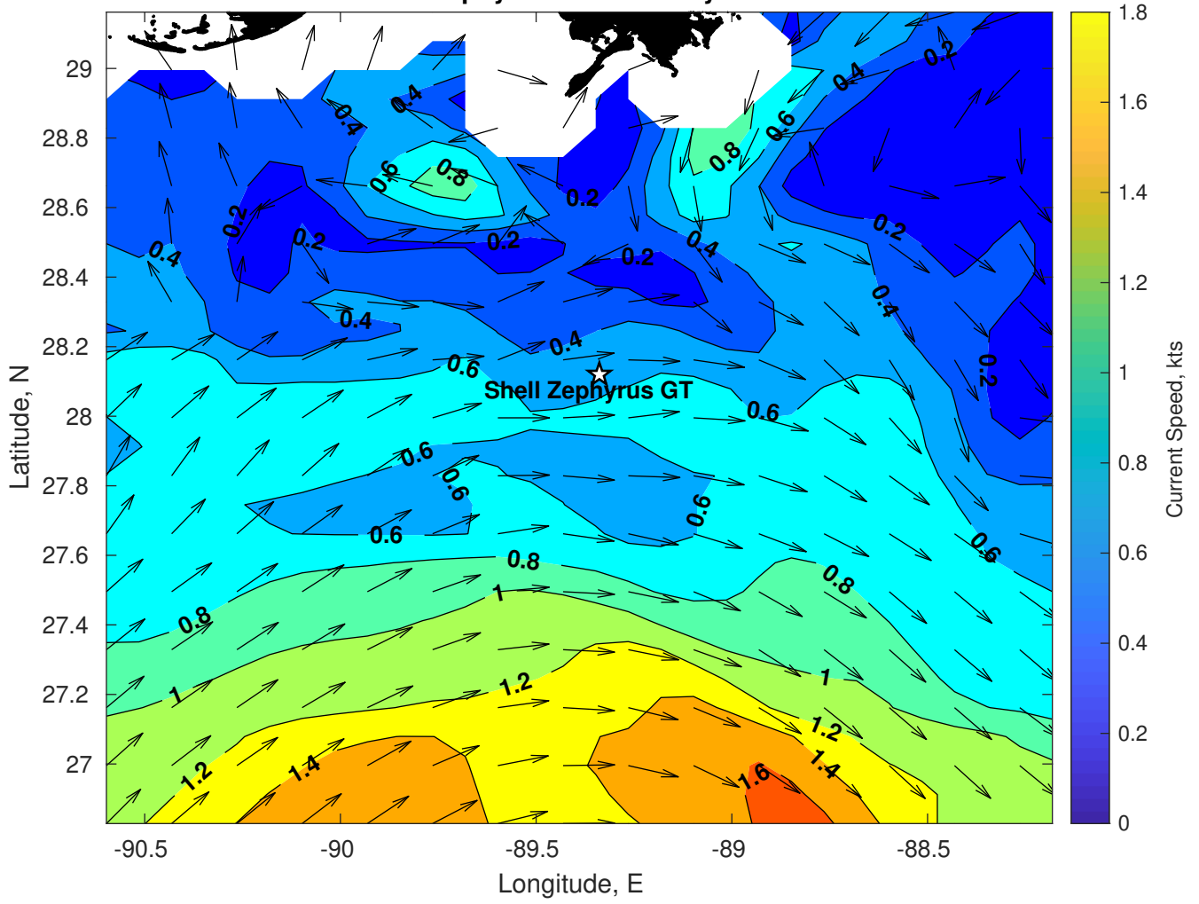
Surface Currents for Shell Zephyrus GT at 09-May-2024 00:00:00
