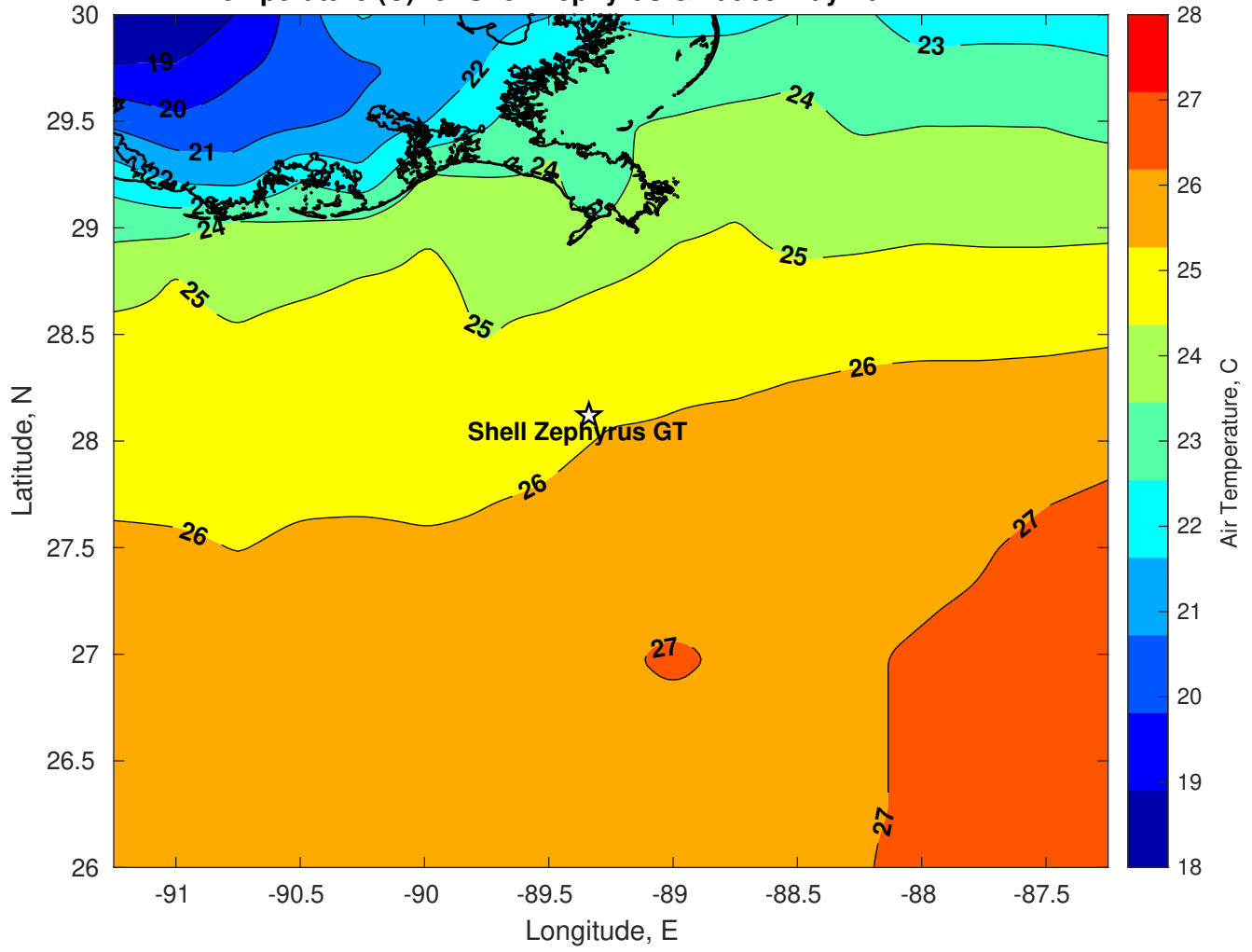
Air Temperature (C) for Shell Zephyrus GT at 09-May-2024
