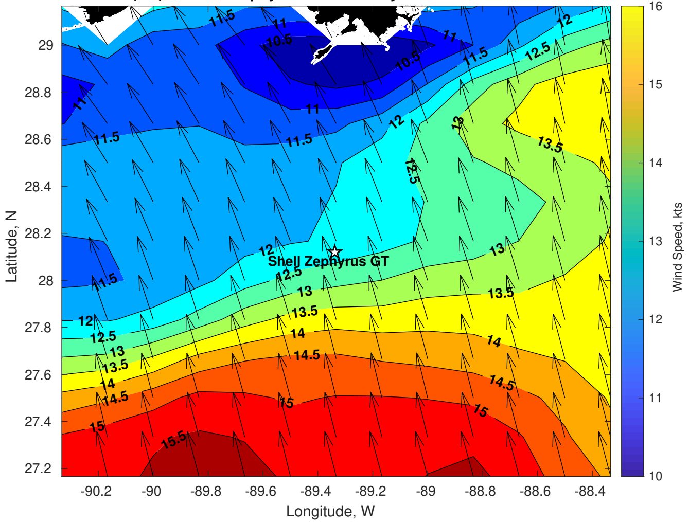
Winds (kts) for Shell Zephyrus GT at 09-May-2024 18:00:00
