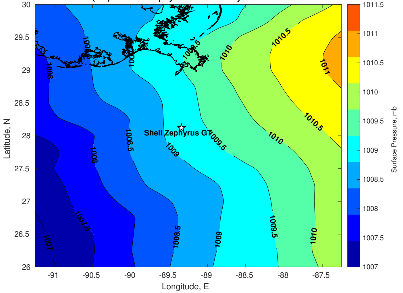
Surface Pressure (mb) for Shell Zephyrus GT at 09-May-2024 12:00:00
