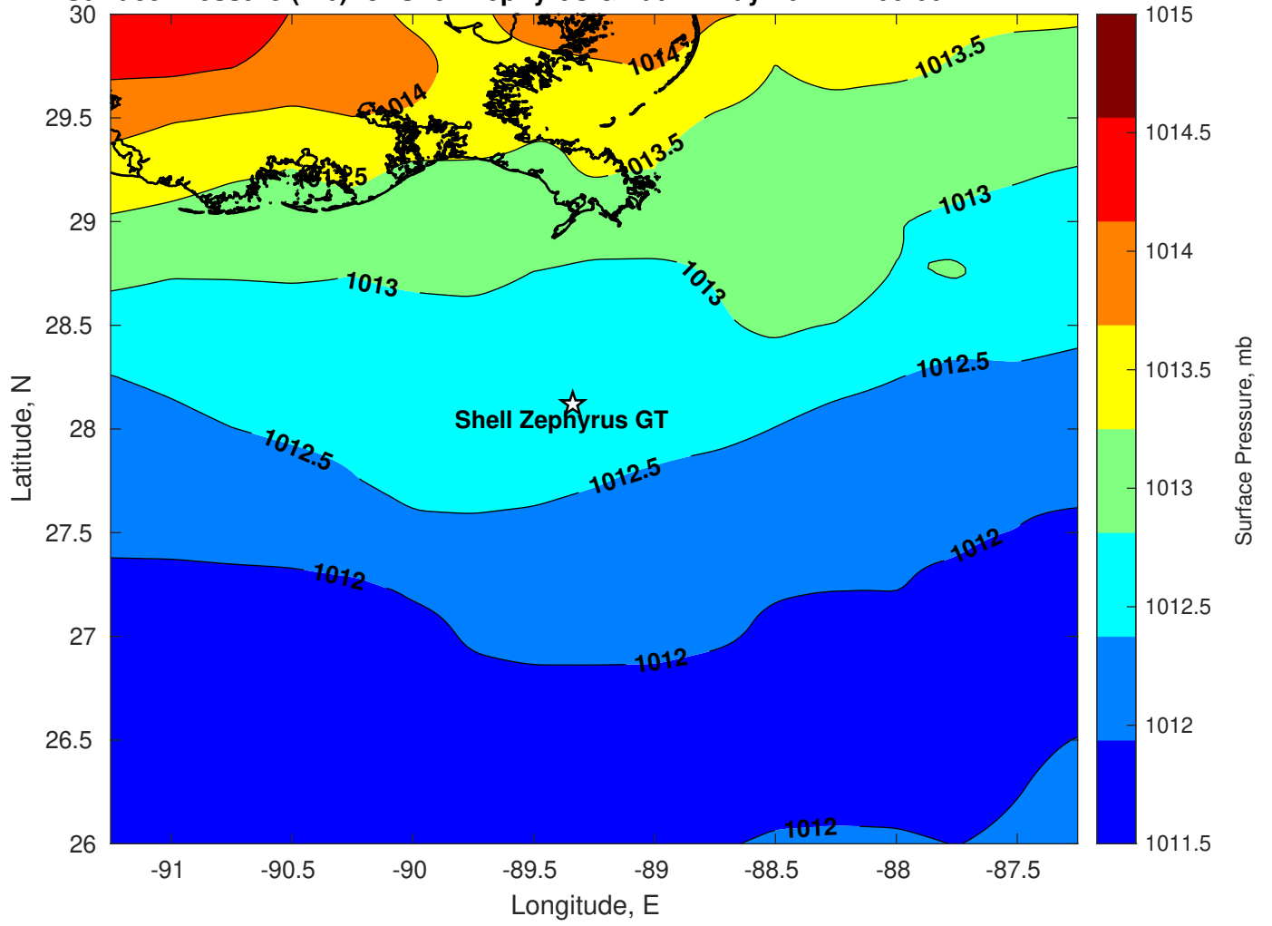
Surface Pressure (mb) for Shell Zephyrus GT at 11-May-2024 12:00:00
