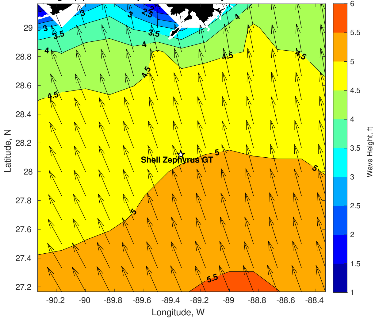
Wave Height (ft) for Shell Zephyrus GT at 09-May-2024 18:00:00
