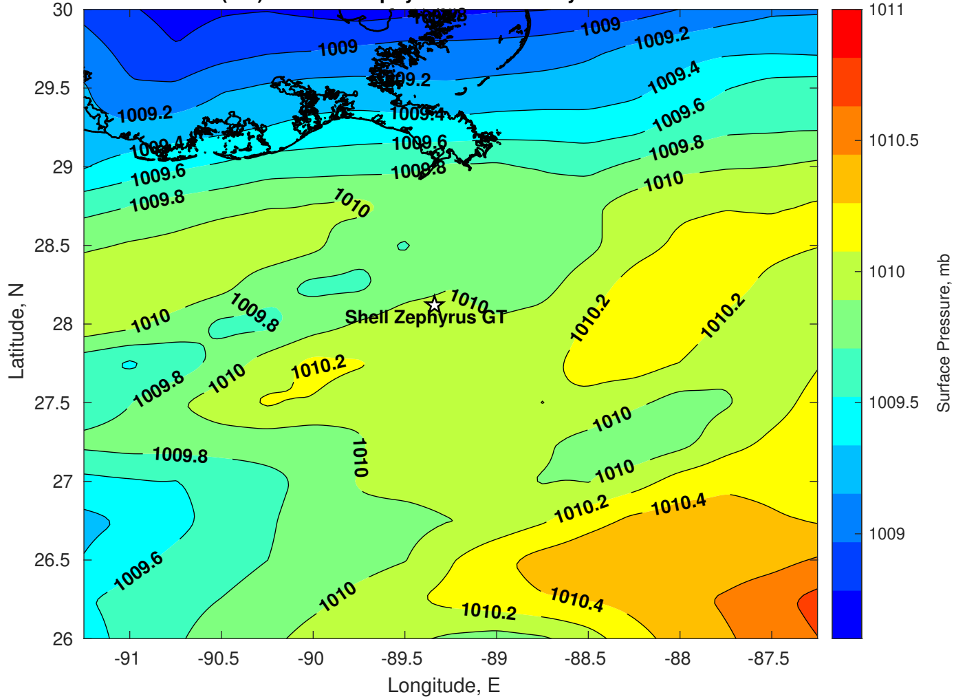
Surface Pressure (mb) for Shell Zephyrus GT at 10-May-2024 12:00:00
