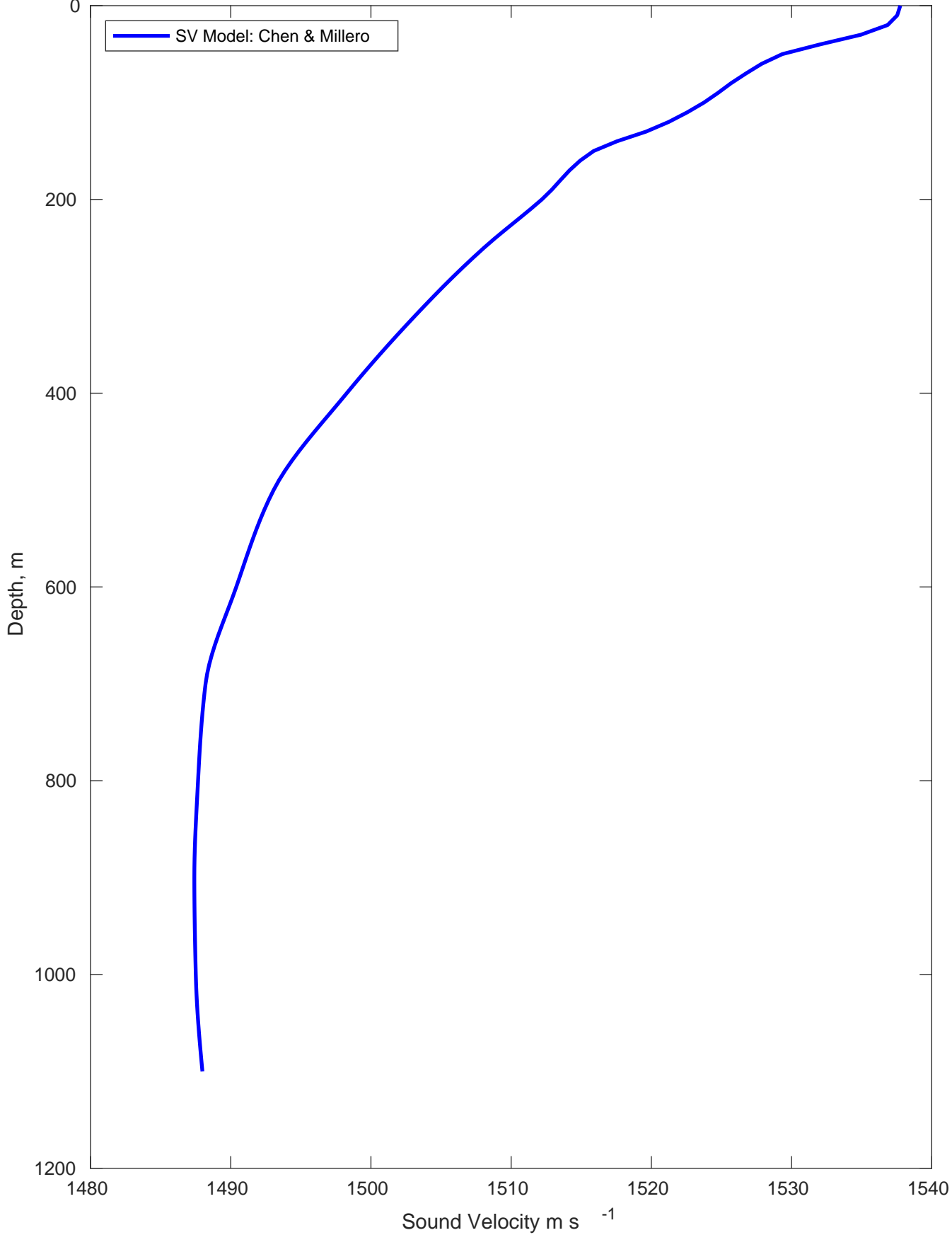
Sound Velocity Profile for Shell Zephyrus GT on 09-May-2024 00:00:00
