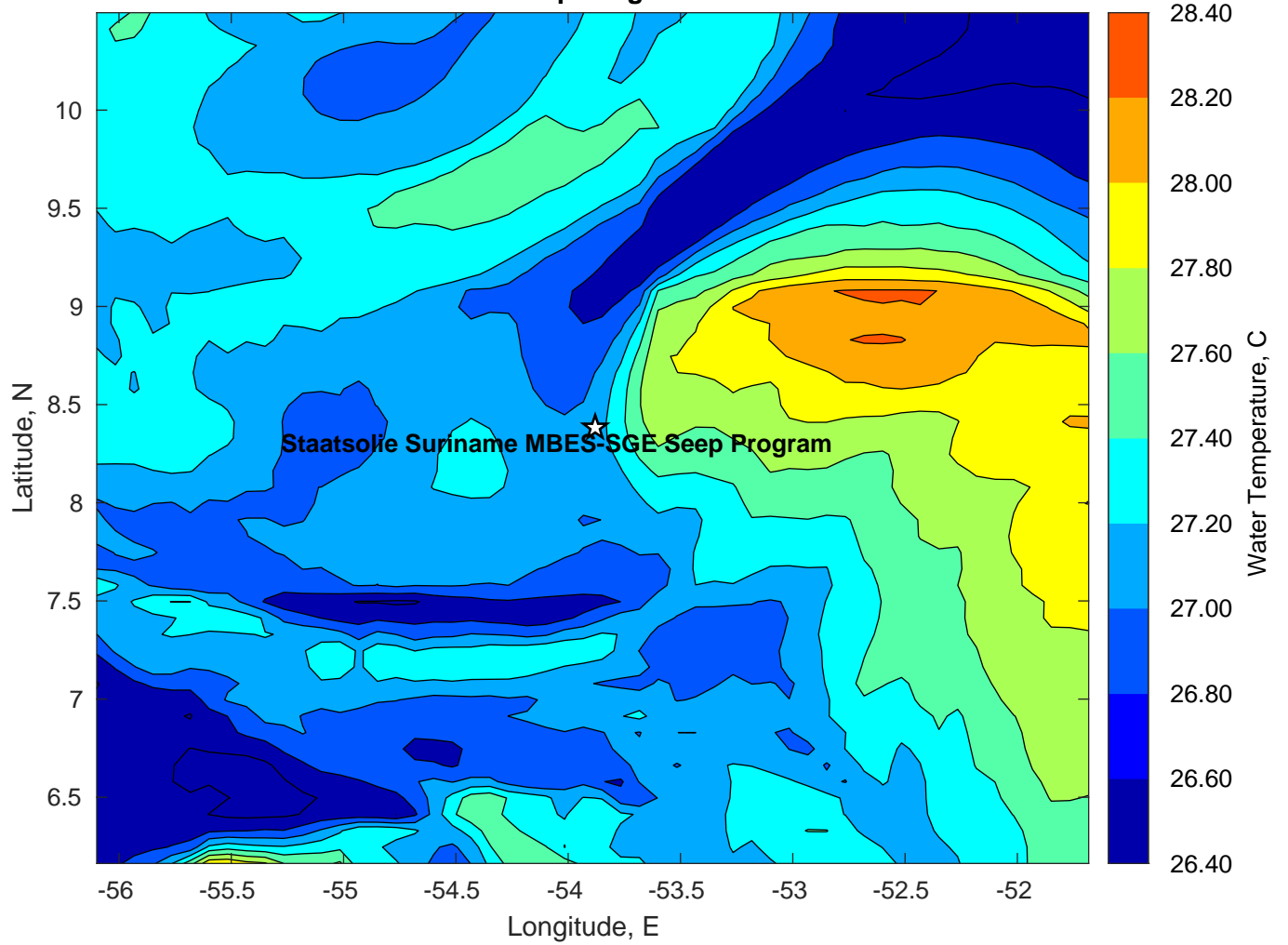
SST for Staatsolie Suriname MBES-SGE Seep Program at 31-Mar-2023 00:00:00
