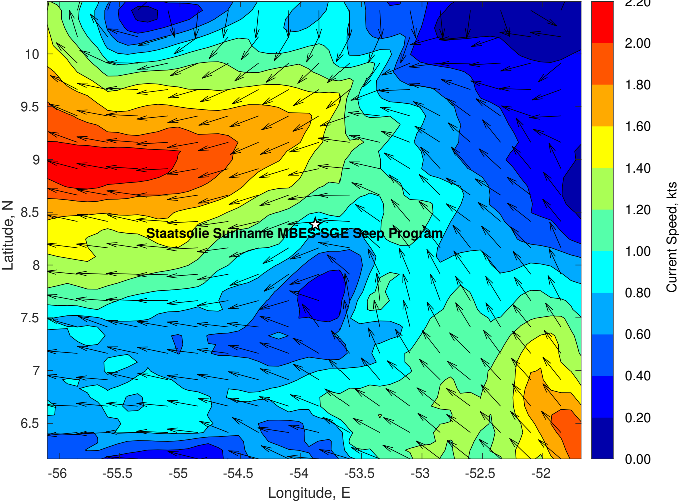
Surface Currents for Staatsolie Suriname MBES-SGE Seep Program at 31-Mar-2023 00:00:00
