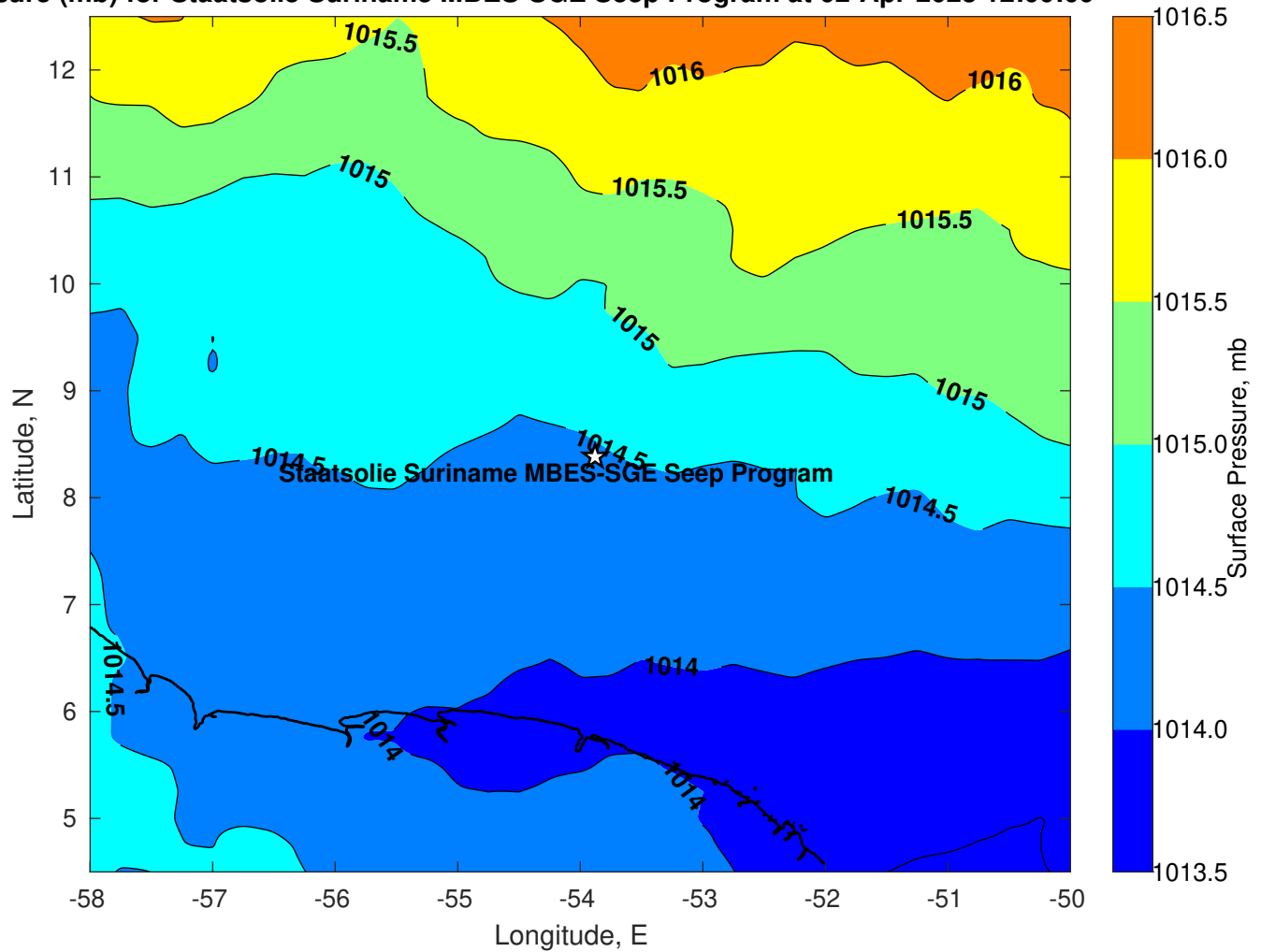
Surface Pressure (mb) for Staatsolie Suriname MBES-SGE Seep Program at 02-Apr-2023 12:00:00
