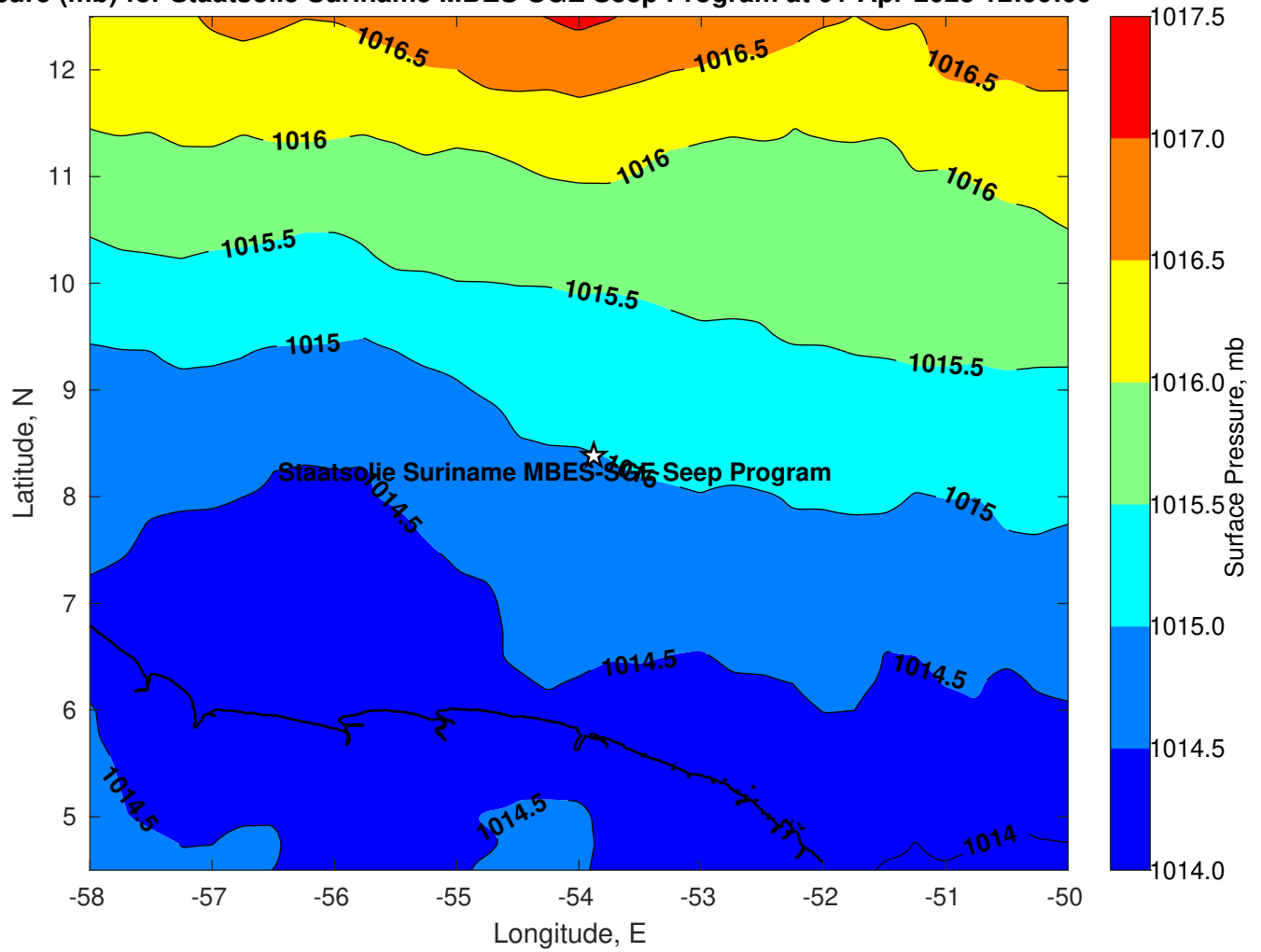
Surface Pressure (mb) for Staatsolie Suriname MBES-SGE Seep Program at 01-Apr-2023 12:00:00
