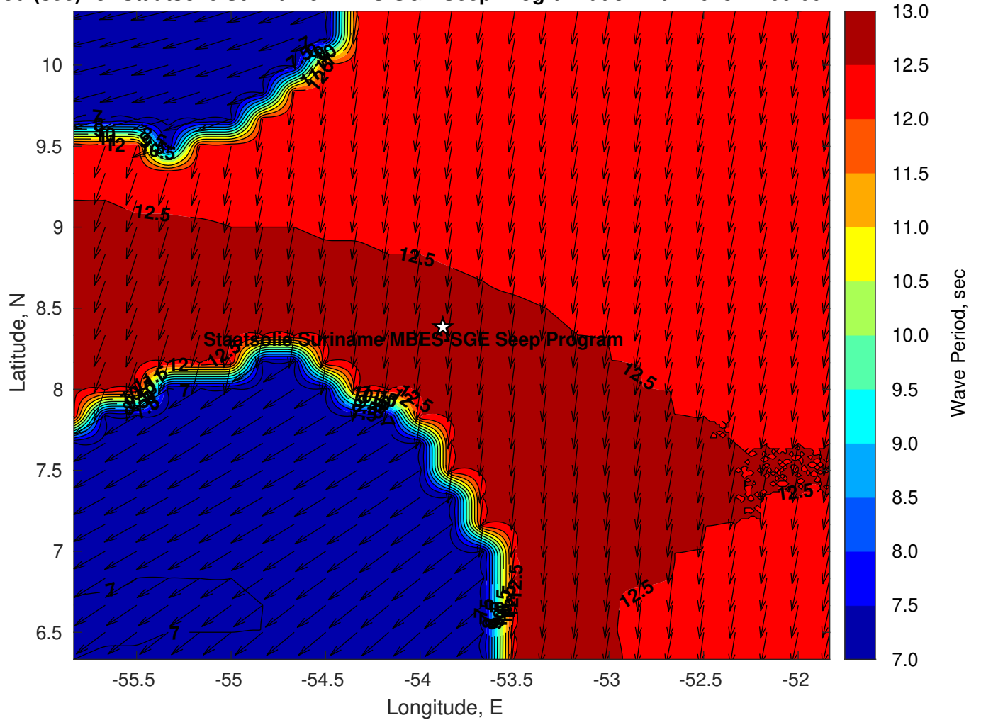
Wave Period (sec) for Staatsolie Suriname MBES-SGE Seep Program at 31-Mar-2023 12:00:00
