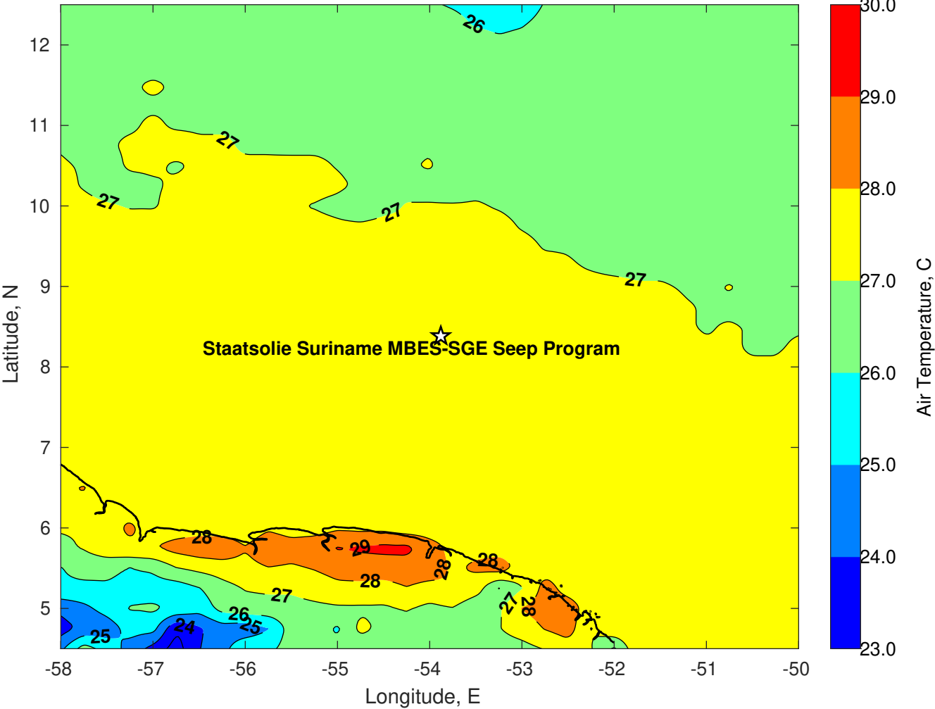
Air Temperature (C) for Staatsolie Suriname MBES-SGE Seep Program at 31-Mar-2023
