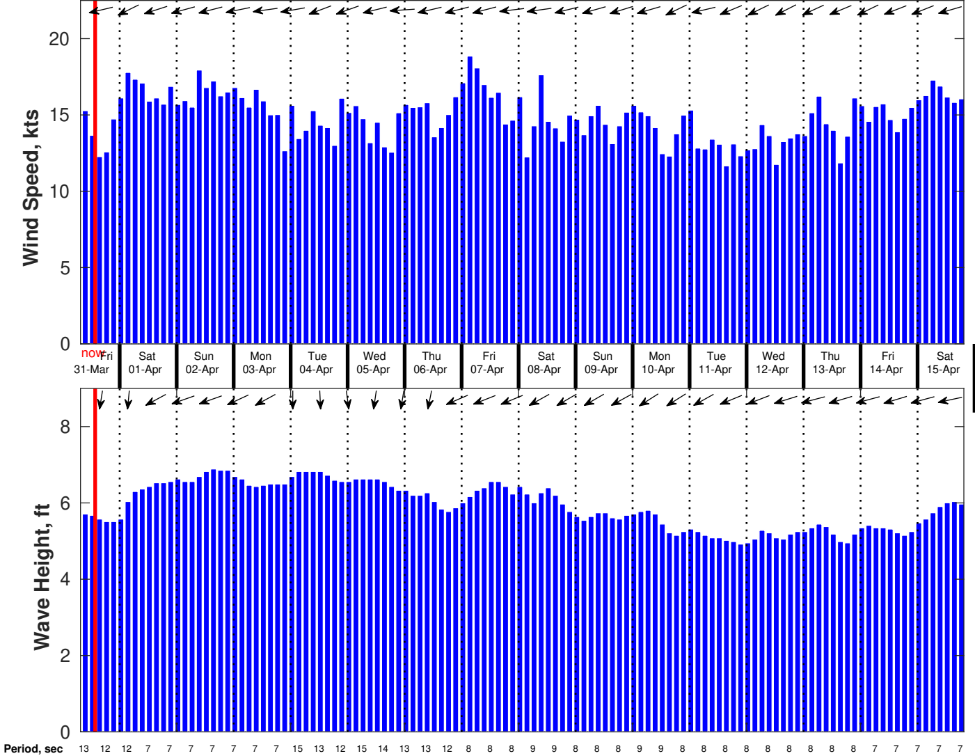
Wind & Wave Forecast for Staatsolie Suriname MBES-SGE Seep Program from 31-Mar-2023 08:00:00 to 16-Apr-2023 08:00:00
