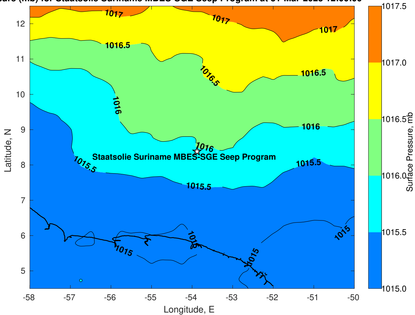
Surface Pressure (mb) for Staatsolie Suriname MBES-SGE Seep Program at 31-Mar-2023 12:00:00
