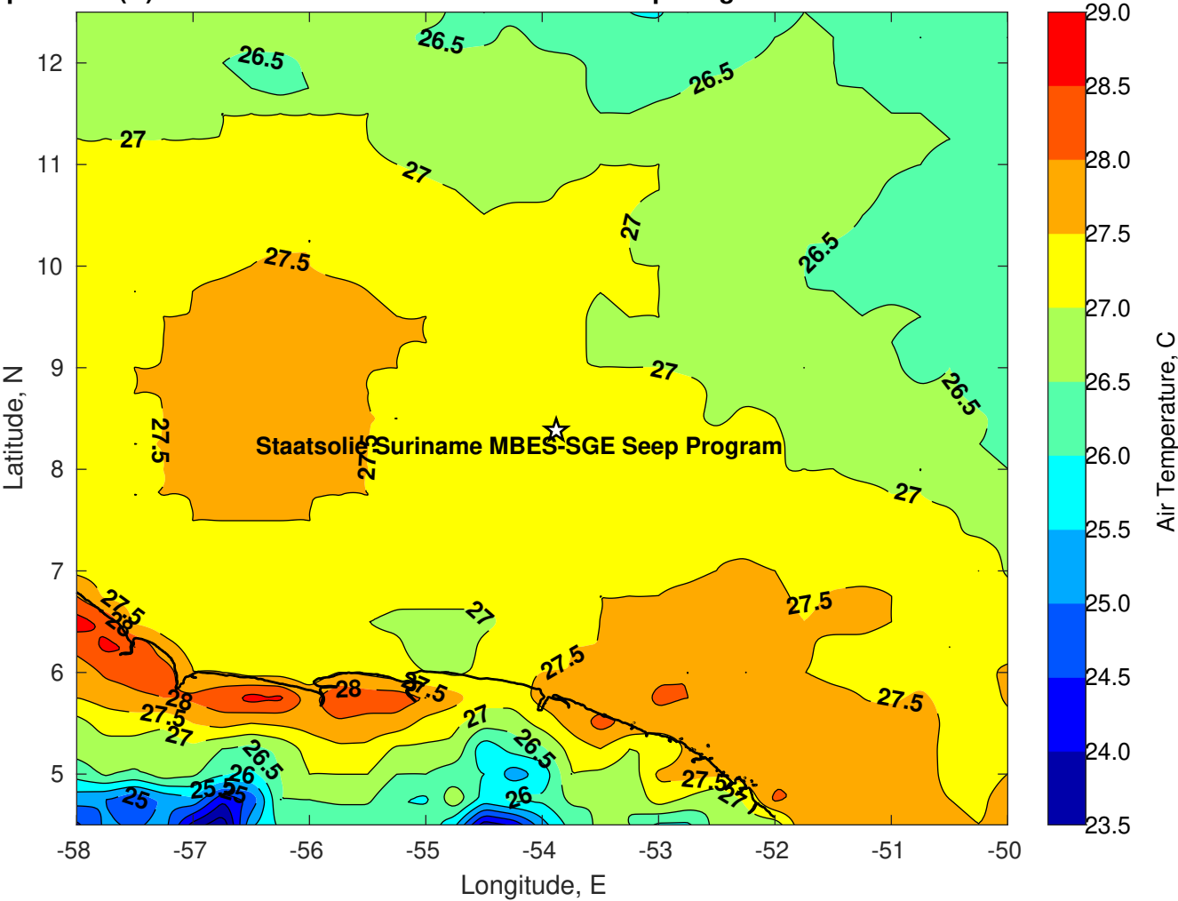
Air Temperature (C) for Staatsolie Suriname MBES-SGE Seep Program at 31-Mar-2023
