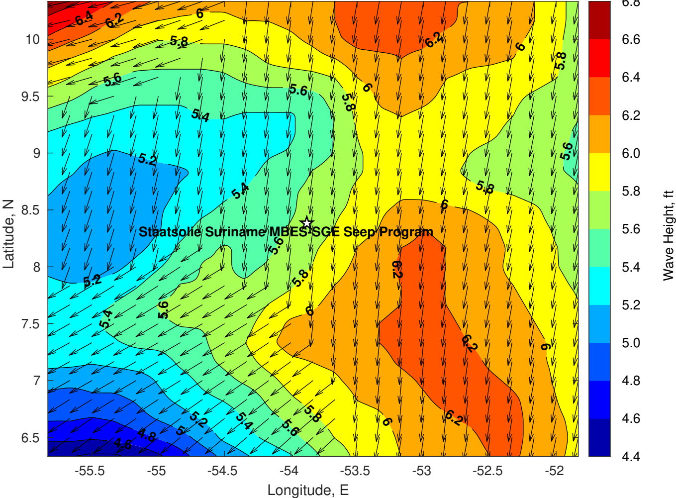
Wave Height (ft) for Staatsolie Suriname MBES-SGE Seep Program at 31-Mar-2023 12:00:00
