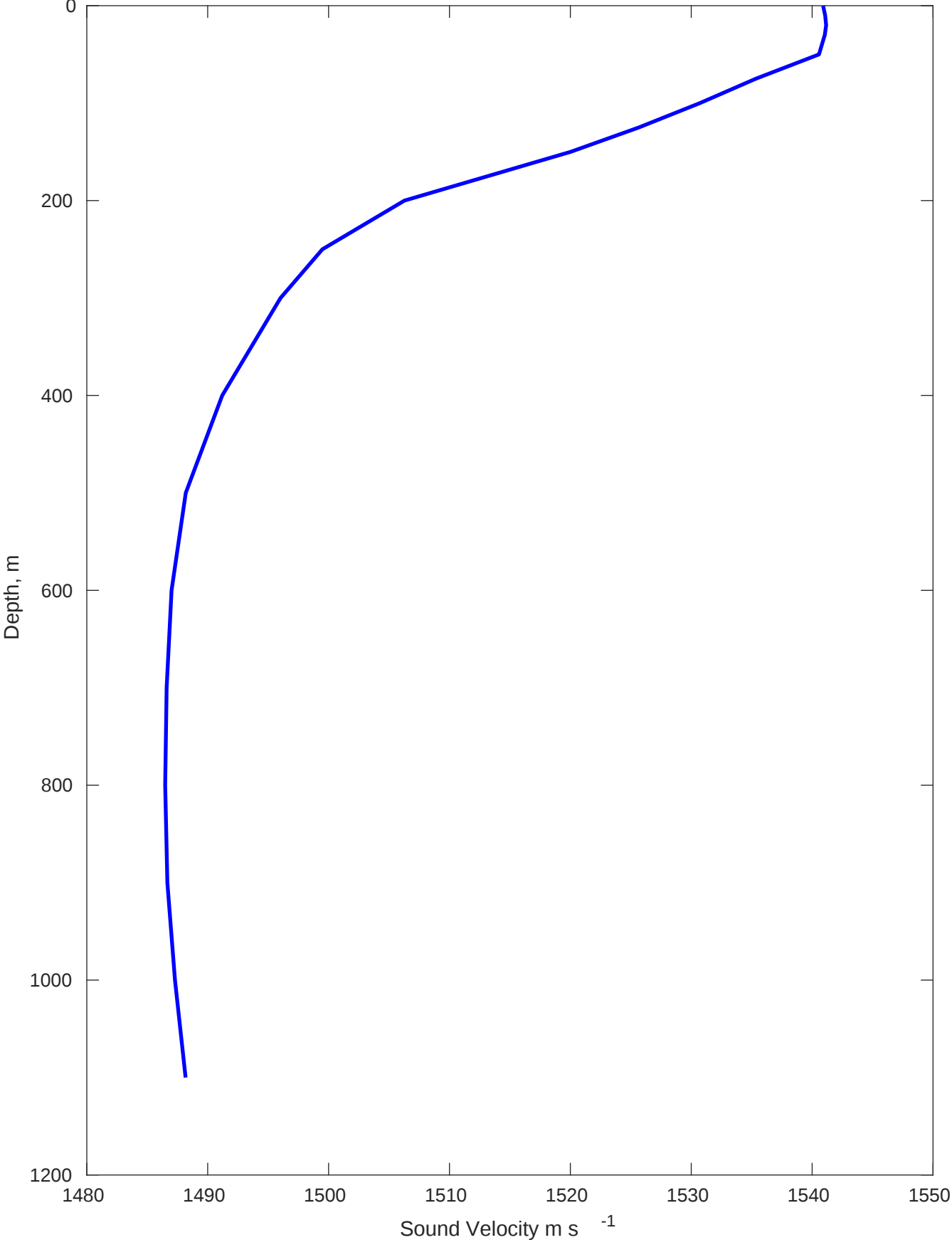
Sound Velocity Profile for Staatsolie Suriname MBES-SGE Seep Program on 31-Mar-2023 00:00:00
