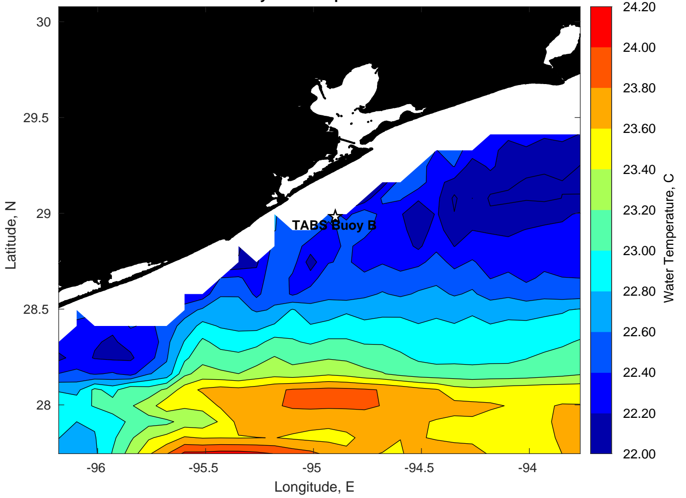
SST for TABS Buoy B at 04-Apr-2023 00:00:00
