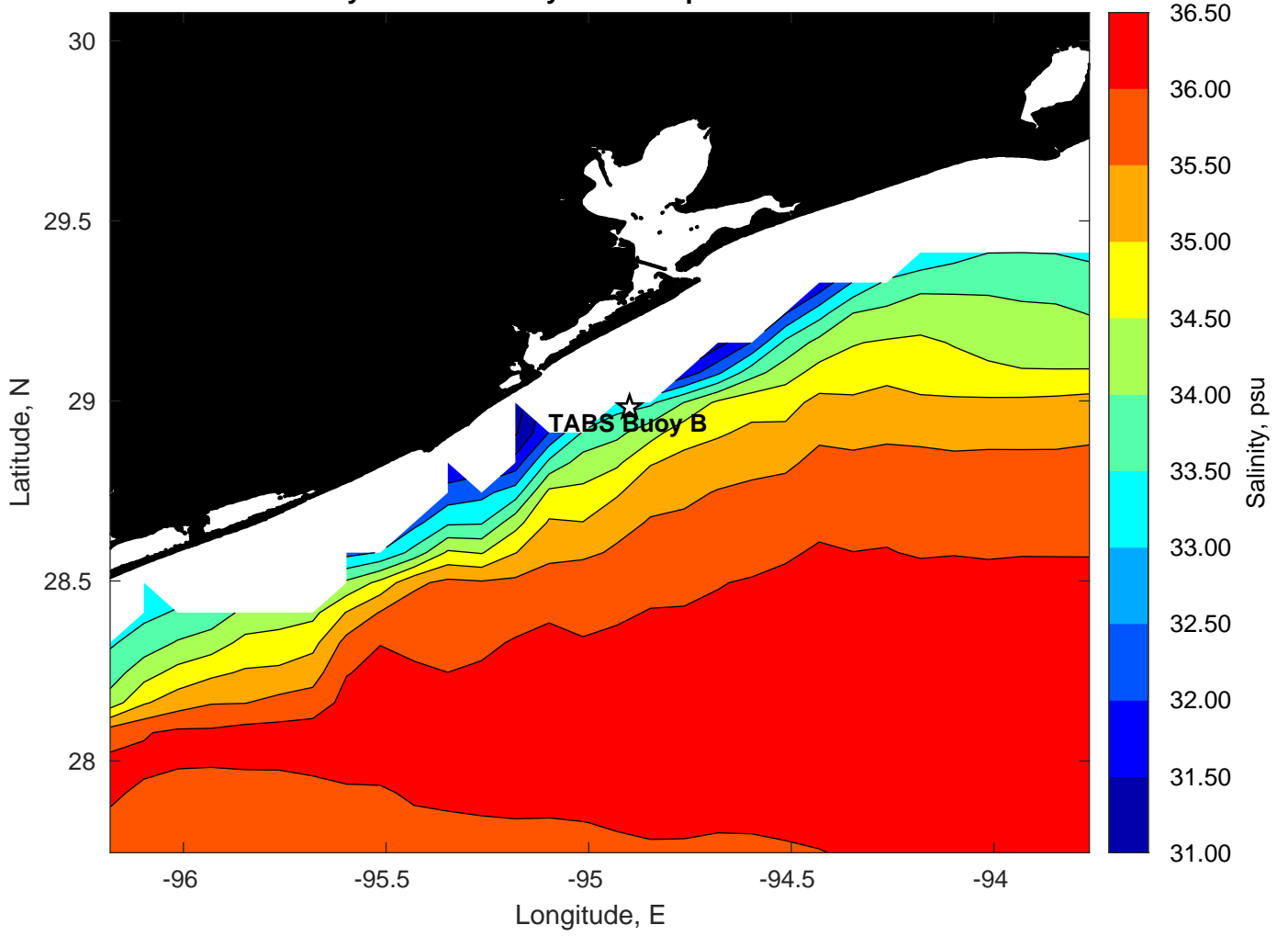
Surface Salinity for TABS Buoy B at 04-Apr-2023 00:00:00
