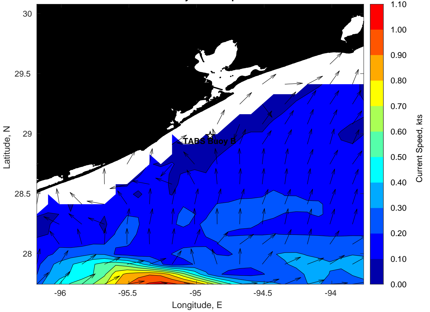
Surface Currents for TABS Buoy B at 04-Apr-2023 00:00:00
